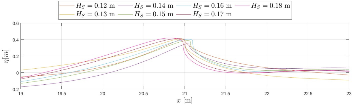
Figure 3.4 – Free-surface profiles of the breaking waves listed in table 3.1 at the instant of breaking. The breaking locations have been iteratively modified.
