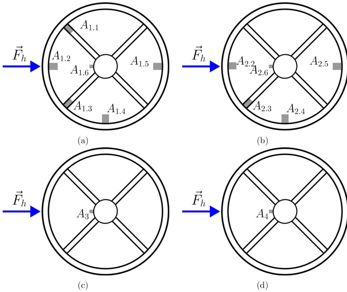
Figure 2.26 – Accelerometer configuration for the complete set-up: top view of the skin elements for sections S_1 (a), S_2 (b), S_3 (c) and S_4 (d).
