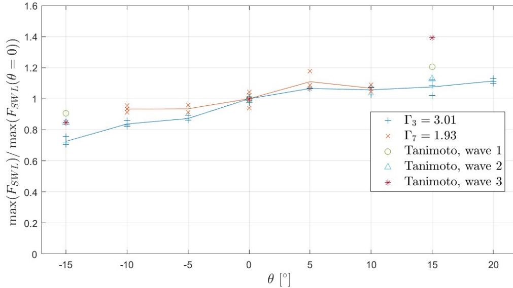
Figure 4.25 – Evolution of the non-dimensionalized maximum impact force as a function of the pitch angle \theta for waves 3 and 7.
