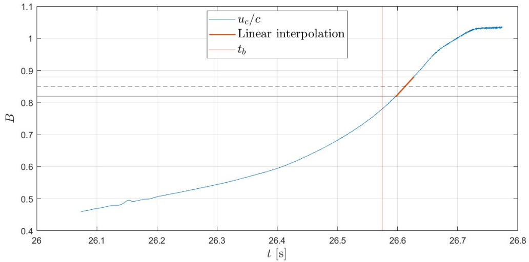
Figure 3.23 – Evolution of parameter B = \frac{u_c}{c} for wave 11.
