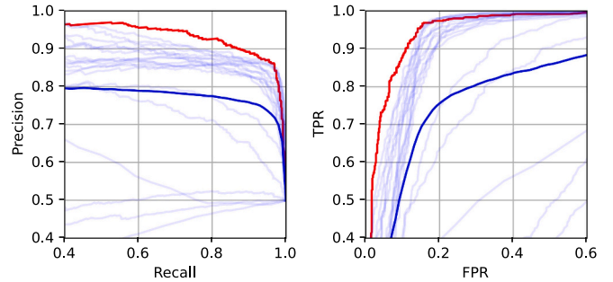
(b) Blue whale's Dcall
