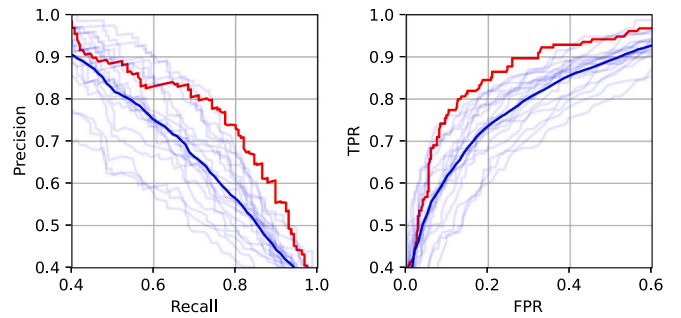
(a) SEIO PBW vocalizations
