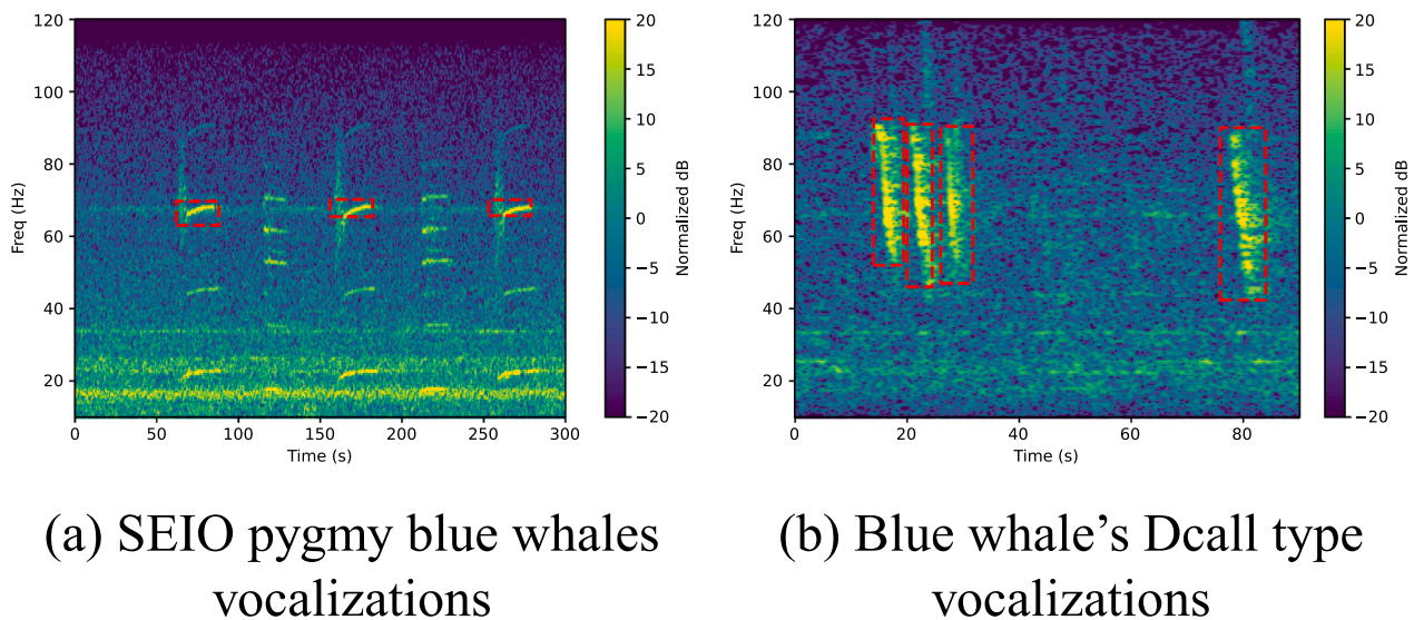
Fig. 2. Spectrograms of the two blue whale's vocalizations annotated during the campaign. Red dotted rectangles correspond to the annotation of the expert. (For interpretation of the references to colour in this figure legend, the reader is referred to the web version of this article.)
