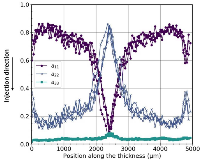
Fig 2. Distribution of the diagonal components of the fiber orientation tensor along the thickness of four samples taken at different positions in two plates.
