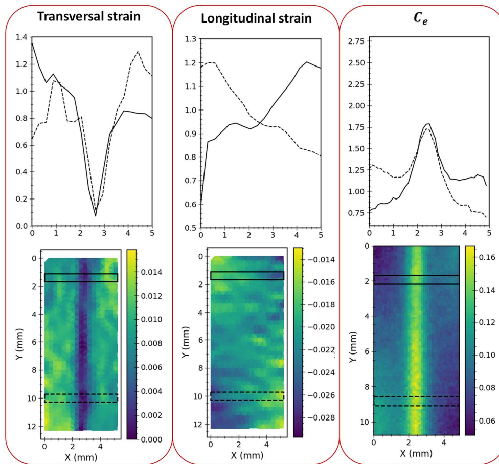
Fig 7. Case of a compression test considered as non-uniaxial: transverse strain field (left), longitudinal strain field (middle), and thermo-elastic coupling field (right), with the associated normalized profiles along the thickness for a normalized maximum stress level in absolute value of 0.86 ( X and Y correspond to the sample thickness and length, respectively; the loading is applied along Y ).
