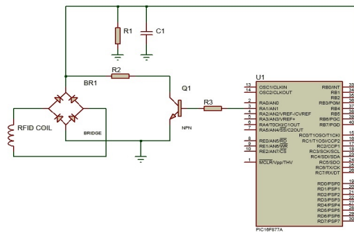
Figure 7: RFID card emulator using PIC16F877A microcontroller
