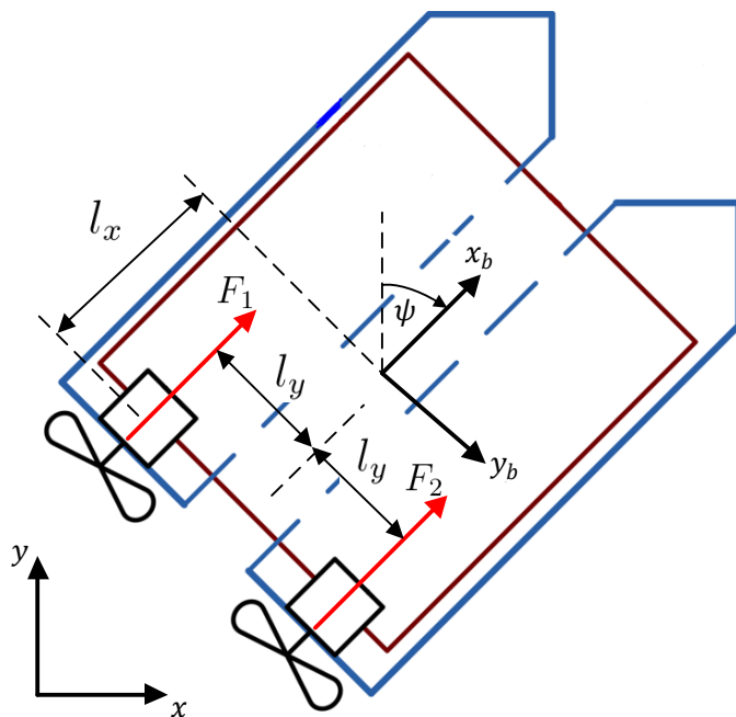
Figure 1. Earth- and body-fixed coordinate systems for the definition of state variables of a USV.
