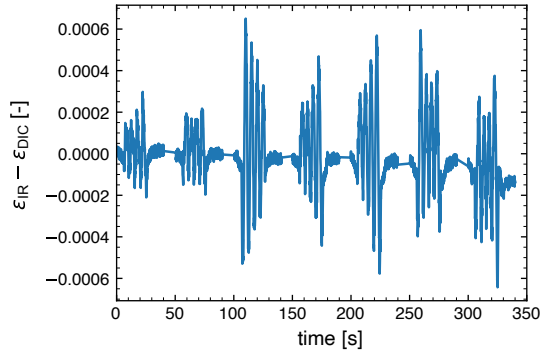
Fig. 8 Difference between the average longitudinal deformation computed by marker detection and DIC.
