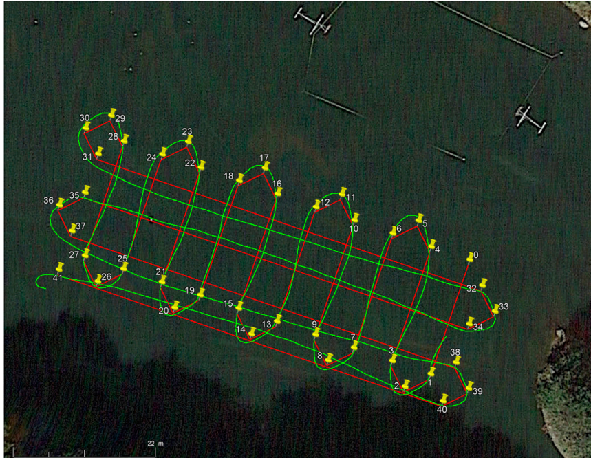
FIGURE 10 | The real boustrophedon track (in green) with the desired waypoints (in yellow, connected by red lines). Short legs are approximately 20 m and long ones are 70 m.
