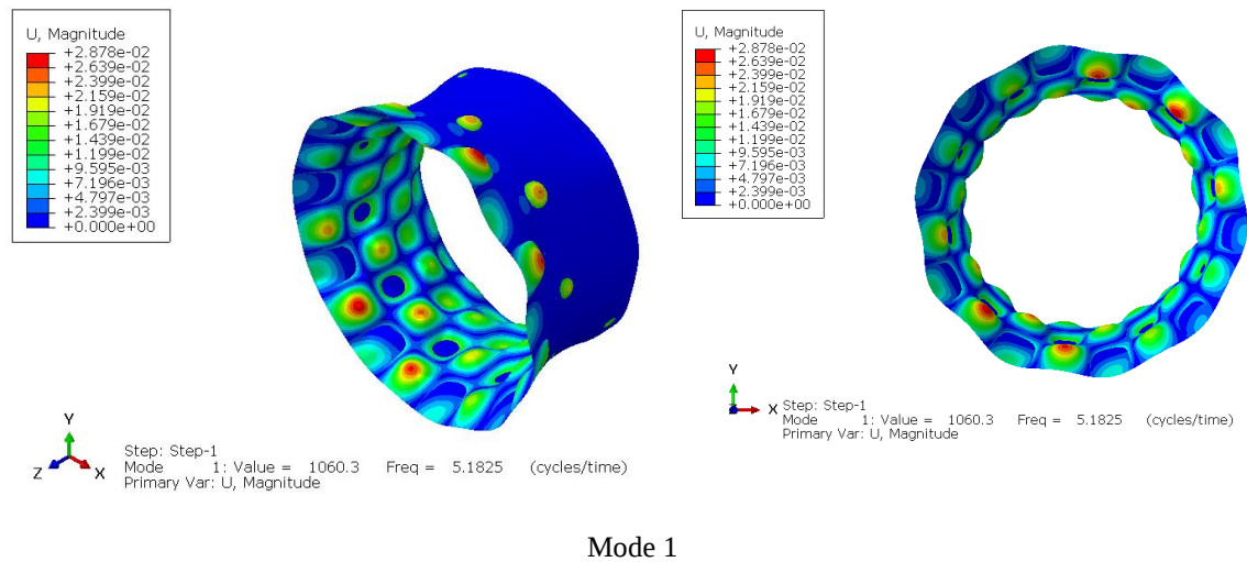
Fig. 10: Natural frequency mode of CGG laminate
