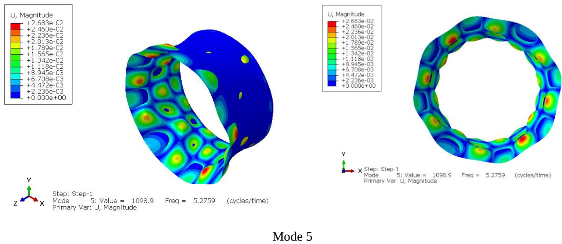
Fig. 10: Natural frequency mode of CGG laminate
