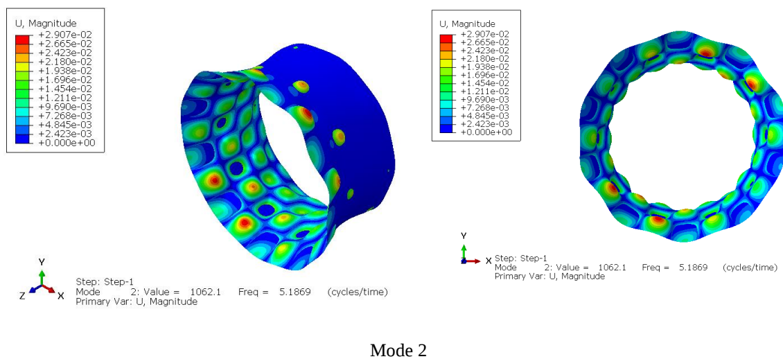
Fig. 11: Natural frequency modes of GGG laminate (contd.)
