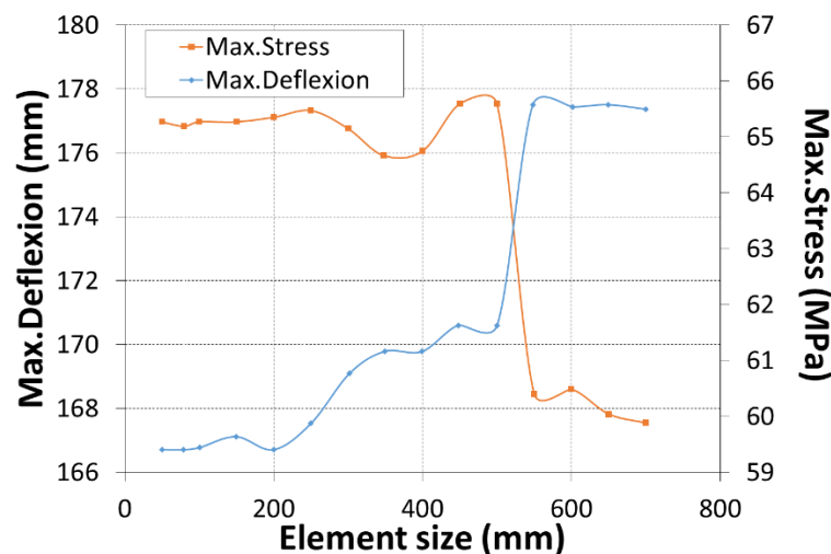
Fig. 6: Mesh convergence
