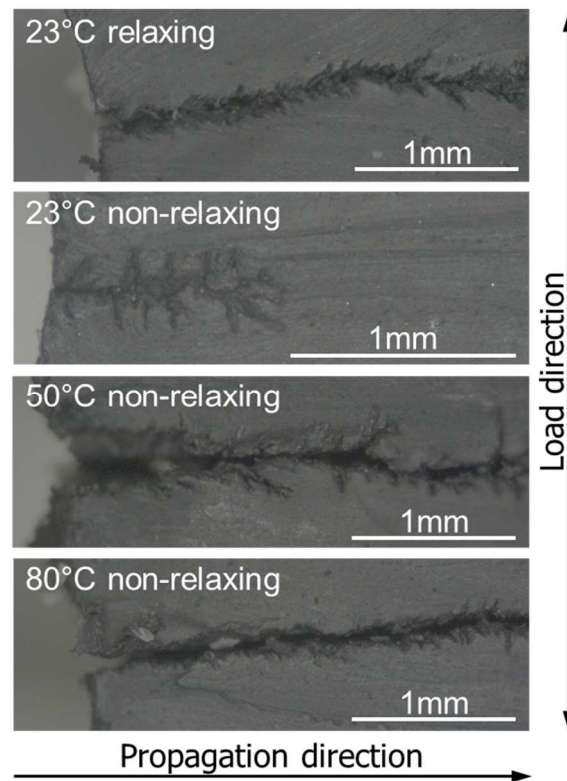
Figure 16: Crack propagation paths for relaxing and non-relaxing load conditions. All shown cracks come from AE2 samples which were loaded in pure tension. The maximum displacement level is 10.6mm for all cracks. Non-relaxing cracks come from minimum displacement levels of 2.65mm.
