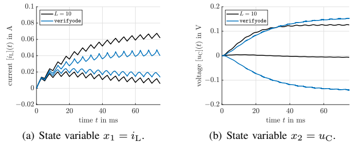
Fig. 6. Comparison between verifyode and the approach from Sec. III-A ( L = 10 ).
