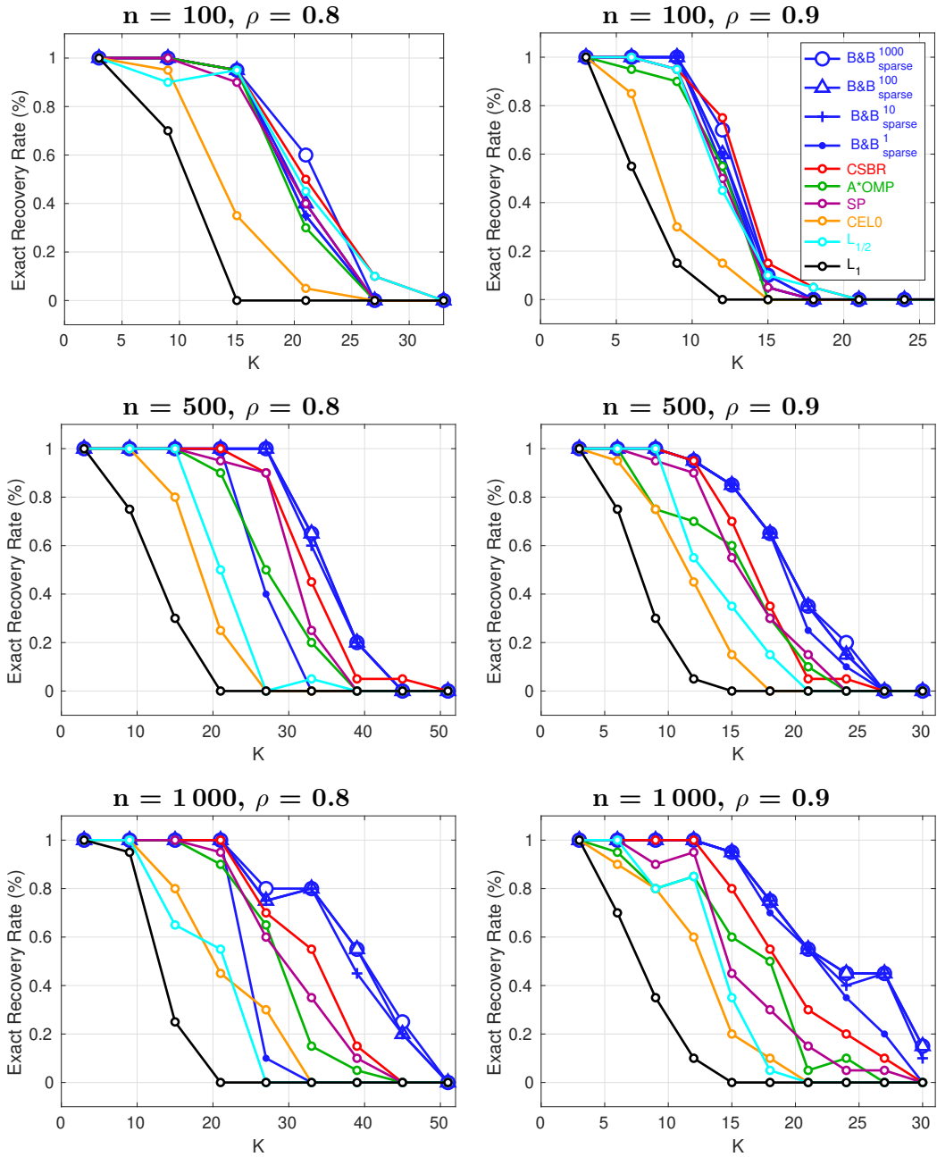
Figure 3. Quality of solutions obtained by B\&B_{sparse} by limiting the computation time to 1, 10, 100 and 1000 s, compared to other state-of-the-art sparse estimation methods: exact recovery rate as a function of the cardinality of the solution for medium (left) and high (right) correlation levels of the columns of \mathbf{A} , and for problems involving n = 100 (top), n = 500 (center) and n = 1000 (bottom) variables. Results are averaged over 20 instances.
