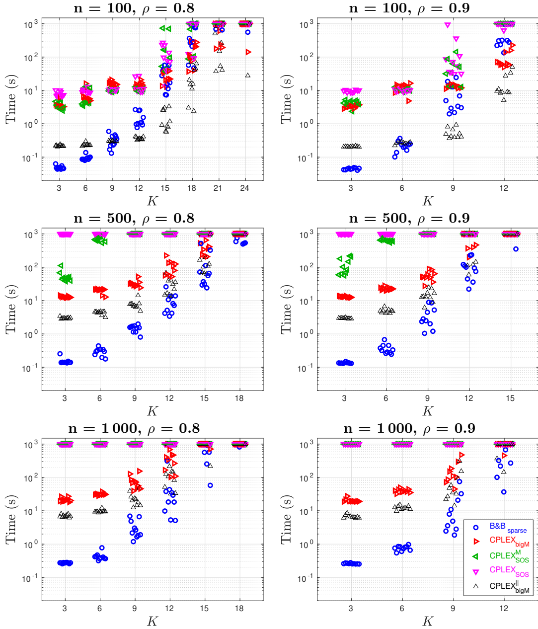
Figure 4. Exact optimization of \mathcal{P}_{2/0} : computation times for B&B sparse and for different MIP formulations solved with CPLEX as a function of the solution cardinality, for medium (left) and high (right) correlation levels \rho of the columns of \mathbf{A} , and for problems involving n = 100 (top), n = 500 (center) and n = 1000 (bottom) variables. Each marker corresponds to one instance, and points are split horizontally around the corresponding cardinality level.
