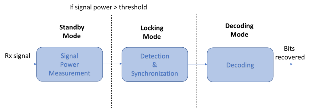
Figure 9. Receiver modes.
