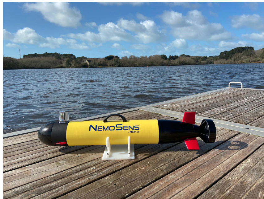
Figure 2. AUV NemoSens.
