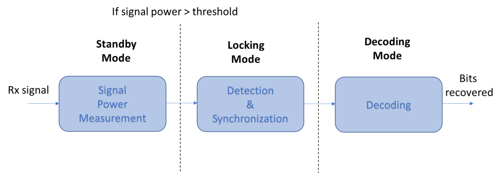
Figure 9. Receiver modes.
