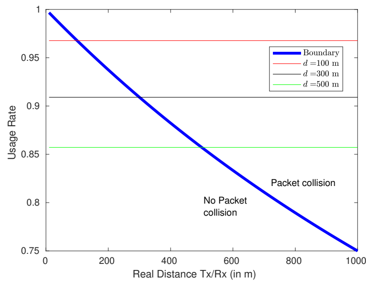
Figure 6. Network usage rate for T_{frame} = 2 s.
