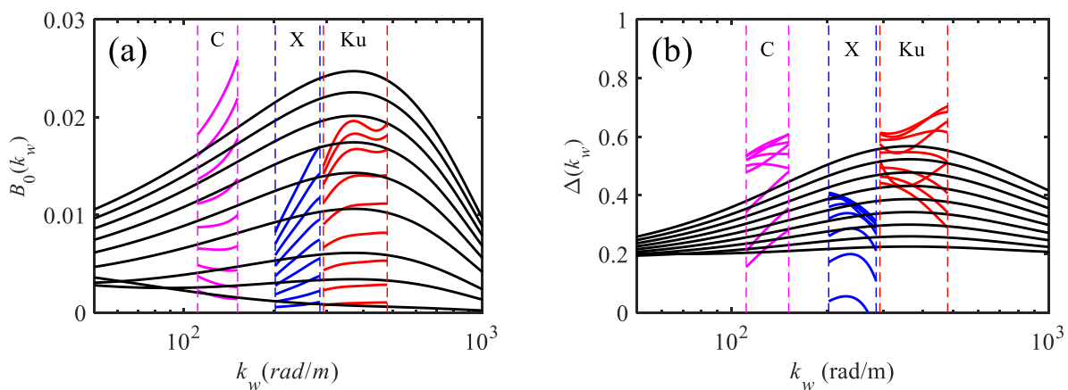
Figure 2. The inverted “pure” Bragg wave spectrum is compared with the E spectrum as wind speed ranges from 3 m/s to 21m/s with a 2 m/s step. (a) The omni-directional part of the curvature spectrum, and (b) the term \Delta(k_w) in spreading function. The purple, blue, and red curves correspond to the region of C-, X-, and Ku-bands.
