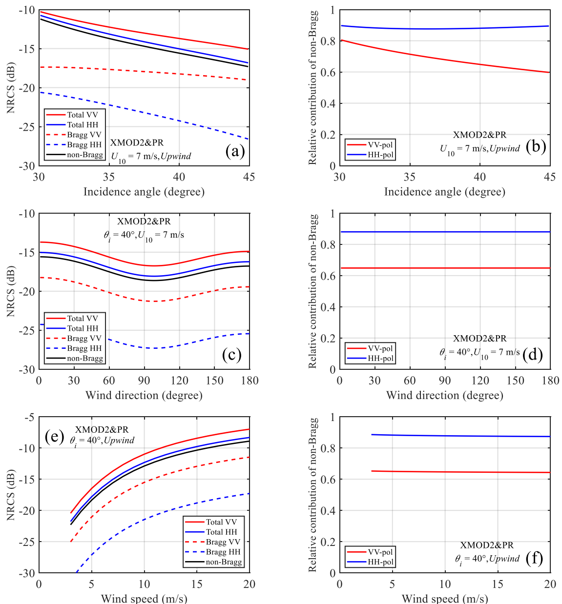
Figure 4. The NRCSs of total scattering, “pure” Bragg wave scattering and non-Bragg scattering, and the relative contribution of non-Bragg scattering estimated by using the XMOD2 and PR model. (a,b): with respect to incidence angles, (c,d) with respect to wind directions, (e,f): with respect to wind speeds.
