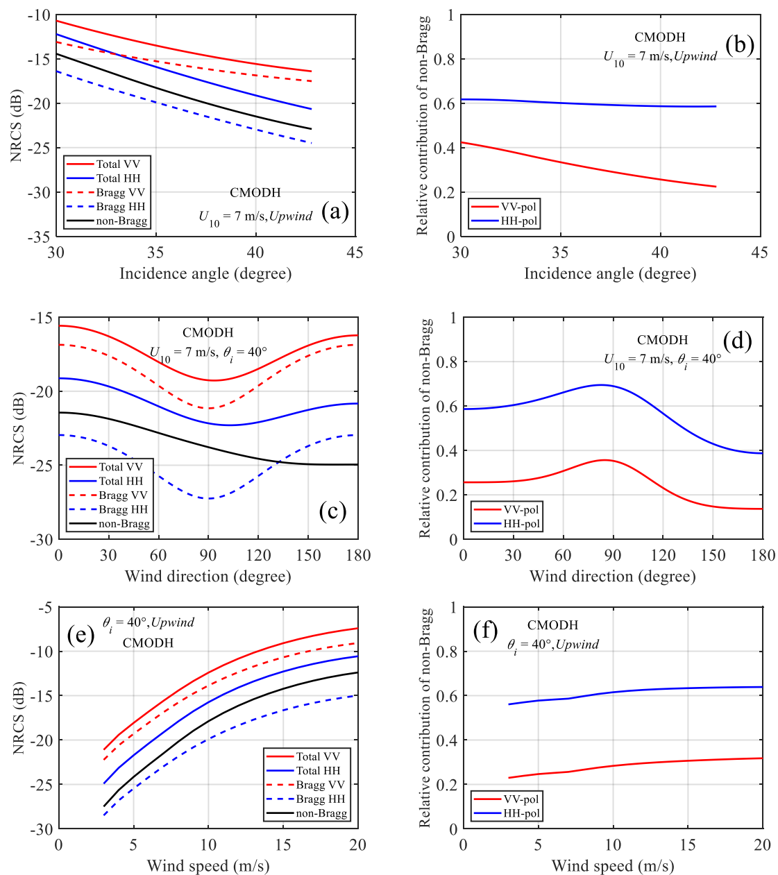
Figure 3. The NRCSs of total scattering, “pure” Bragg wave scattering and non-Bragg scattering, and the relative contribution of non-Bragg scattering estimated by using the CMODH. (a,b): with respect to incidence angles, (c,d): with respect to wind directions, (e,f): with respect to wind speeds.
