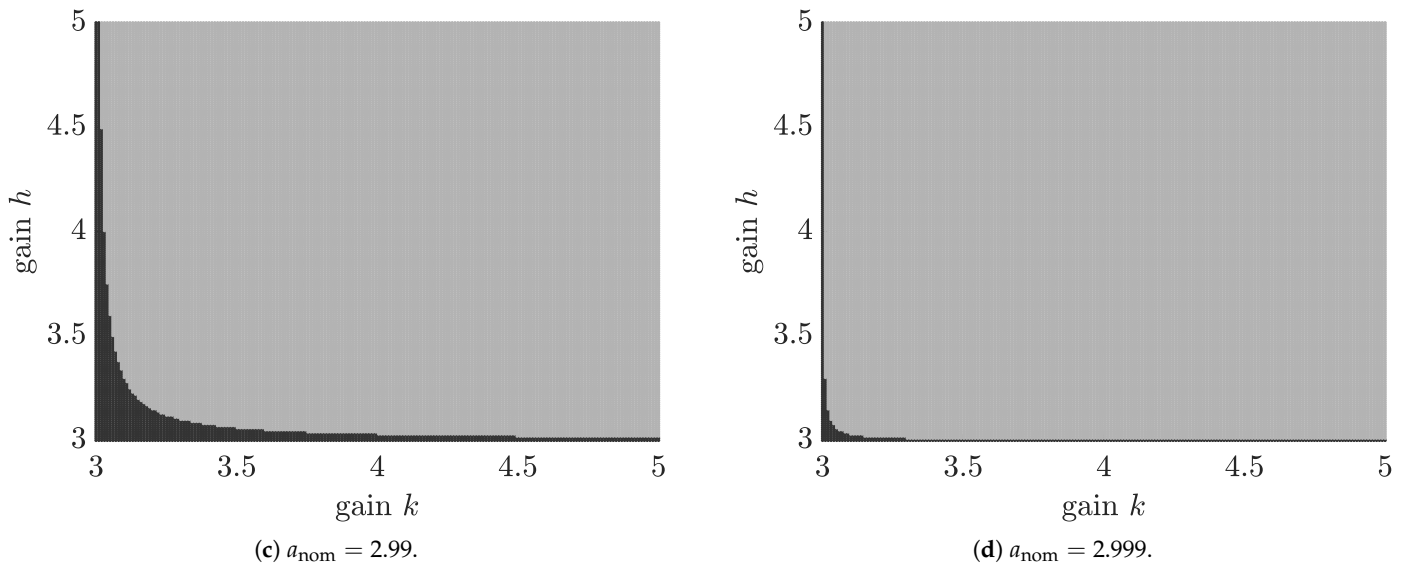
Figure 1. Stability analysis of the observer-based closed-loop control system (7) for different values of a_{\text{nom}} and a \in [1 ; 3] : The choice of a_{\text{nom}} \neq \bar{a} requires a significant increase of both k and h above the thresholds k > 3 and h > 3 .
