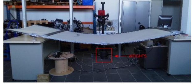
Figure 11 Picture of GP5 panel under loading: 14.26 kg per battens.
