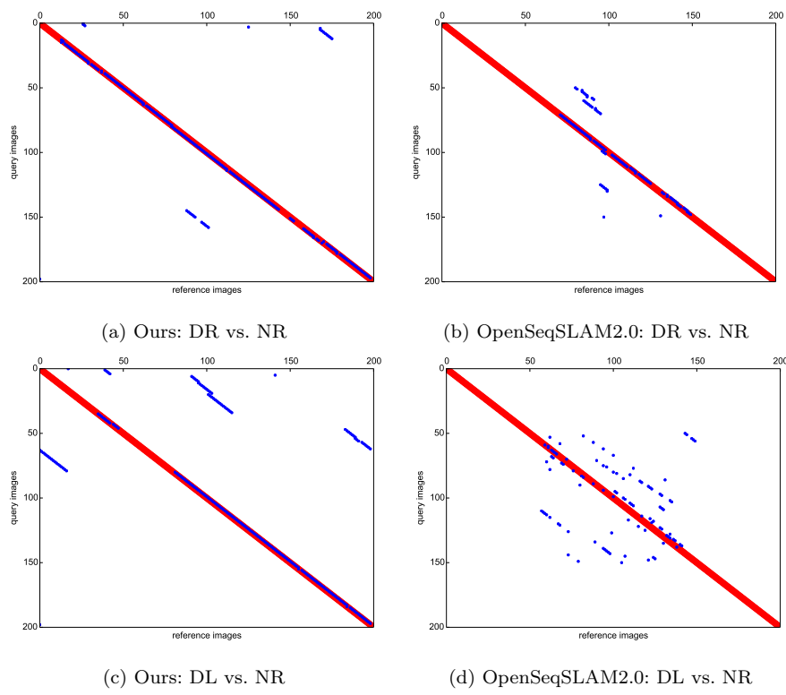
Fig. 19: GPW dataset. Groundtruth and matches are depicted in red and blue, respectively.
