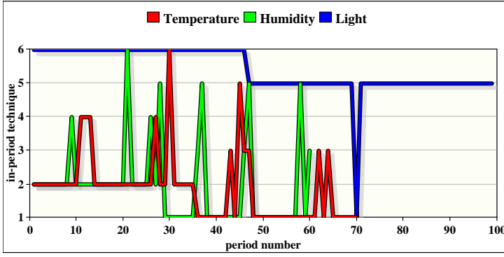
Fig. 5 Variation of the in-period decision made by the sensor at each round, \mathcal{F} = 50 , \delta = 0.1 , \varepsilon = 0.5 , c = 5 .
