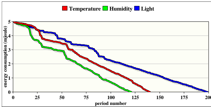
Fig. 8 Remaining energy in a sensor in function of the period progress, \mathcal{F} = 50 , \delta = 0.1 , \varepsilon = 0.5 , c = 5 .
