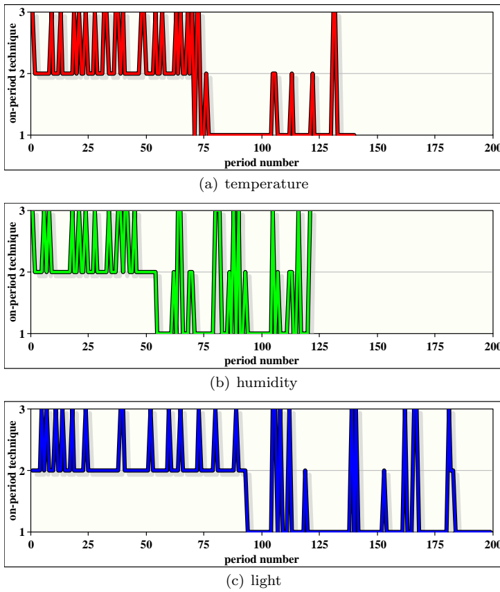
Fig. 4 Variation of the on-period technique selected by the sensor at each period, \mathcal{F} = 50 , \delta = 0.1 , \varepsilon = 0.5 , c = 5 .
