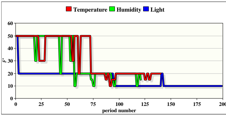
Fig. 6 Variation of the sensing frequency of a sensor during periods, \mathcal{F} = 50 , \delta = 0.1 , \varepsilon = 0.5 , c = 5 .
