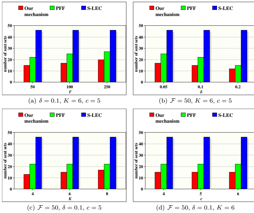
Fig. 10 Number of sets sent periodically from the CH to the sink.
