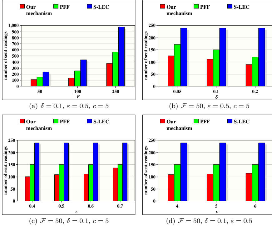
Fig. 7 Number of readings sent from each sensor to the CH.
