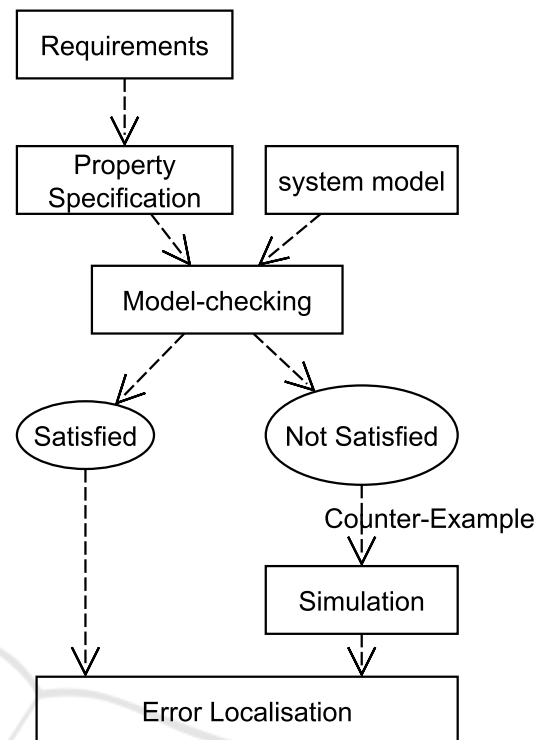
Figure 1: Model-Checking Representation.
