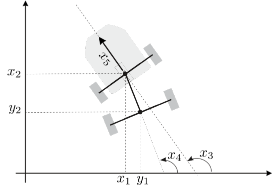
Fig. 1. Tank with a trailer
