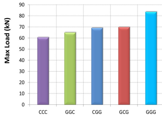
Figure 13. Maximum contact forces of the five configurations.
