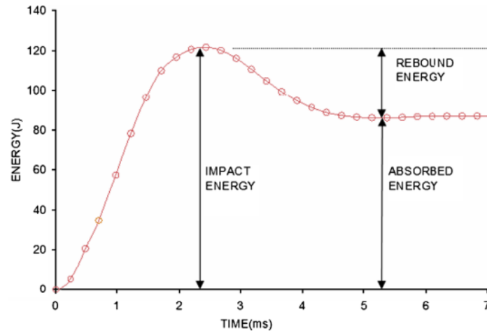
Figure 10. Energy curve in the case of the impactor rebound.
