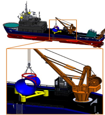
(b) our case of installation of the tidal turbine nozzle
