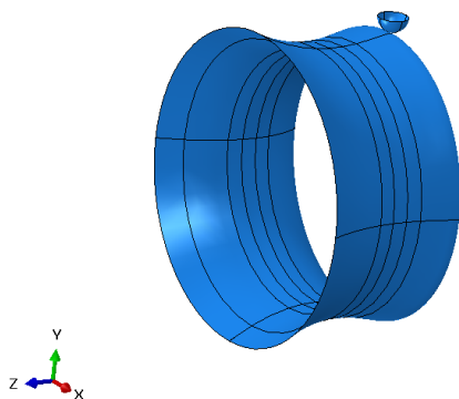
(c) The model of the impactor on the leading edge
