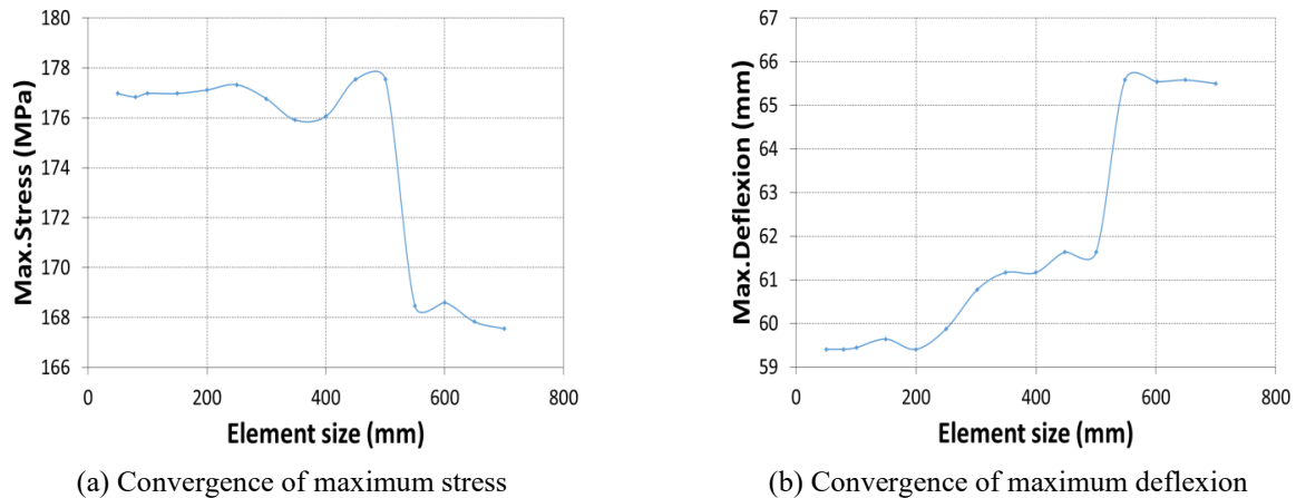
Figure 6. Mesh convergence.
