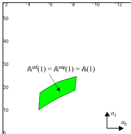
Fig. 28: The CS [[A(1)]] = A(1)
