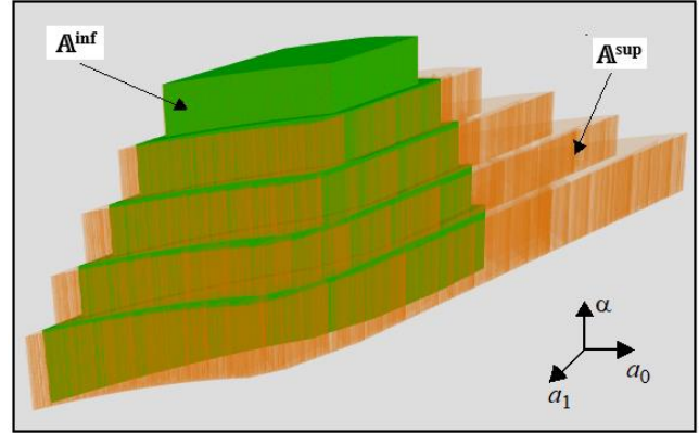
Fig. 29: The TFS [[A]] = [[A^{\text{inf}}, A^{\text{sup}}]]
