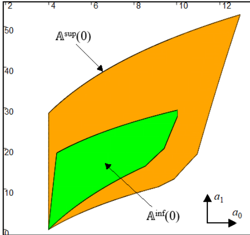
Fig. 27: The TS [[A(0)]] = [[A^{\text{inf}}(0), A^{\text{sup}}(0)]]
