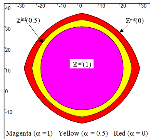
Fig. 17: The lower bounds Z^{inf}(0) , Z^{inf}(0.5) and Z^{inf}(1)
