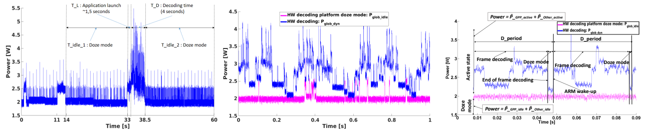
(a) HW video decoding power consumption complete data-logging
