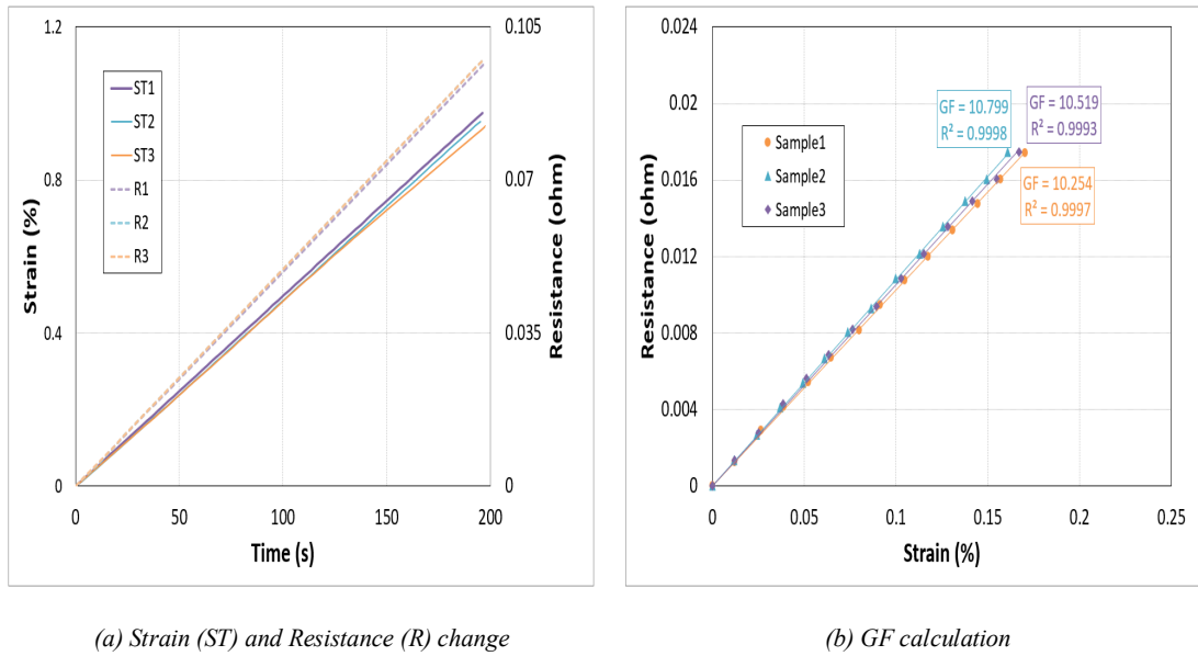
Figure 6: Experimental behavior and calculation of the strain sensitivity of the CF membrane sensor. ST represents the strain of all three samples and R represent the resistance of the sample.
