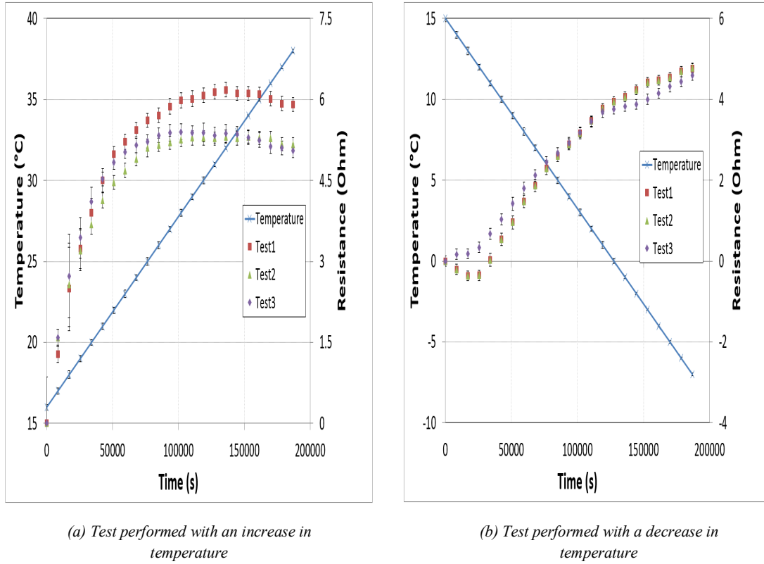
Figure 8: Electrical behavior of CM during thermal loading to detect thermal change.
