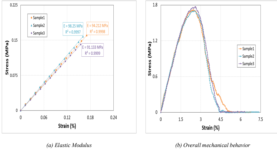
Figure 5: Mechanical performance of the CF sensor.
