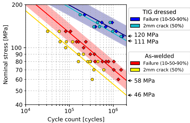
Fig. 21. Conventional fatigue tests results analysed with proposed post-treatment.
