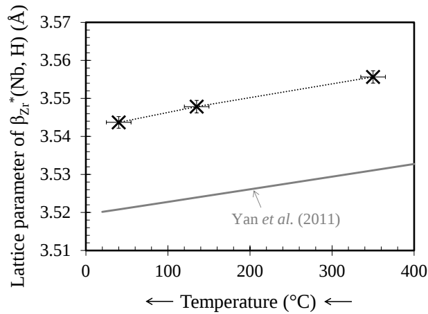
Fig. 9. Evolution of the lattice parameter of the \beta_{Zr}^*(\text{Nb}, \text{H}) phase as a function of temperature obtained by neutron diffraction performed in situ during step-cooling ( 0.01^\circ\text{C/s} on average) from 700^\circ\text{C} on M5 containing about 3300 wppm of hydrogen (and 0.2 wt% of oxygen) water quenched from 1000^\circ\text{C} ; comparison to results from Yan et al. [24].
