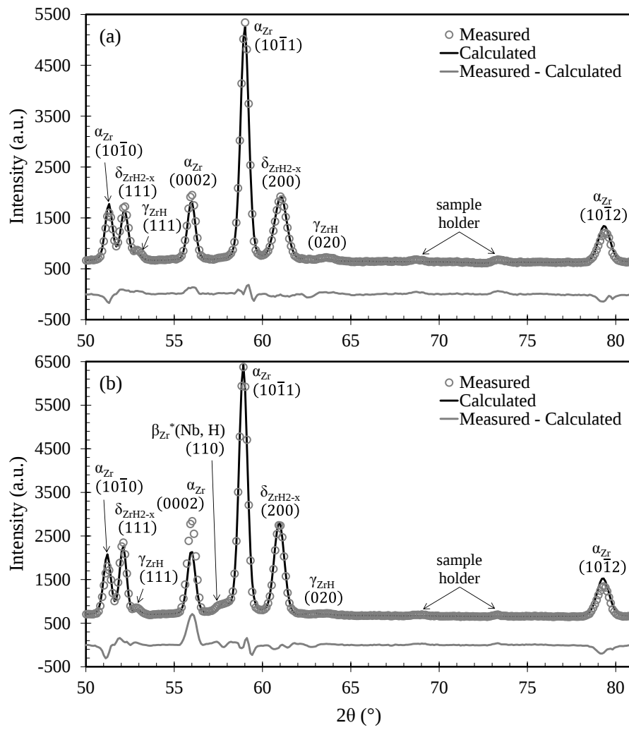
Fig. 4. Rietveld refinement of the neutron diffraction patterns measured at RT after step-cooling (0.01°C/s on average) from 700°C for (a) Zircaloy-4 and (b) M5 containing about 3300 wppm of hydrogen (and 0.2 wt% of oxygen) water quenched from 1000°C.
