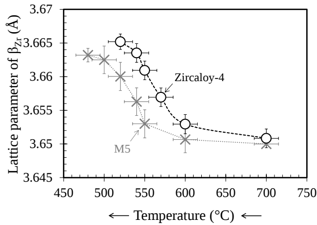
Fig. 8. Evolution of the lattice parameter of the \beta_{Zr} phase as a function of temperature obtained by neutron diffraction performed in situ during step-cooling ( 0.01^\circ\text{C/s} on average) from 700^\circ\text{C} on Zircaloy-4 and M5 containing about 3300 wppm of hydrogen (and 0.2 wt% of oxygen) water quenched from 1000^\circ\text{C} .
