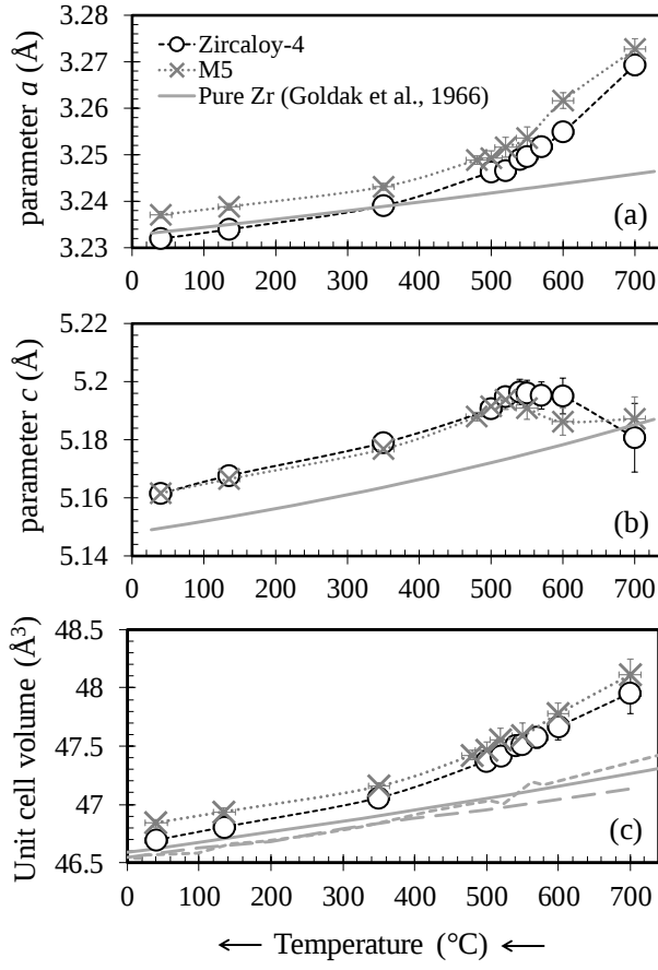
Fig. 7. Evolution of (a) parameter a , (b) parameter c and (c) volume of elementary cell of the \alpha_{\text{Zr}} phase as a function of temperature obtained by neutron diffraction performed in situ during step-cooling ( 0.01^\circ\text{C/s} on average) from 700^\circ\text{C} on Zircaloy-4 and M5 containing about 3300 wppm of hydrogen (and 0.2 wt% of oxygen) water quenched from 1000^\circ\text{C} ; comparison to data reported by Russell [32], Couterne and Cizeron [33] and Goldak et al. [34] for pure zirconium with almost no hydrogen.
