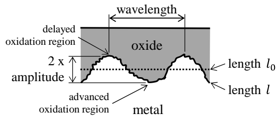
Fig. 14. Schematic representation of the characteristics of the undulations at the metal-oxide interface.
