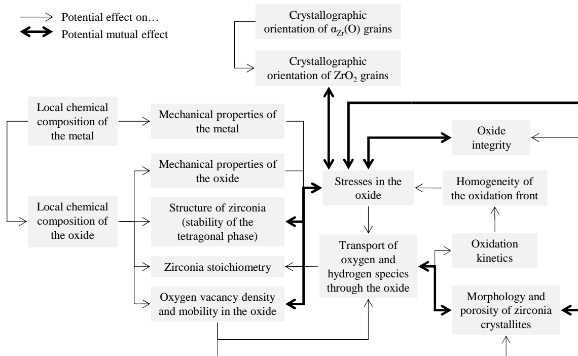
Fig. 24. Factors and properties that may have an effect on breakaway oxidation around 1000°C and potential relationships between them.
