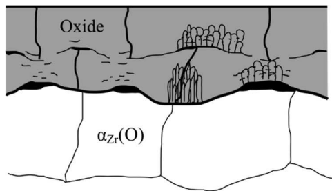
Fig. 20. Schematic representation of the cross-section of the material quenched after breakaway oxidation under steam at 1000°C.
