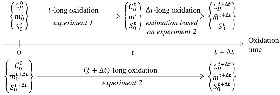
Fig. 7. Parameters used in Eqs. (1) and (2) to calculate the “instantaneous” hydrogen pickup fraction over a time period [t; t + \Delta t] from the data of two experiments performed on samples with different initial mass and surface area.
