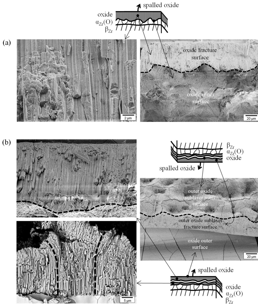
Fig. 18. FEG-SEM fractographs of fragments of oxide spalled during quenching of Zircaloy-4 (batch 1) samples fractured at room temperature after one-side oxidation for (a) 5000 s and (b) 7500 s at 1000°C and water quenching.
