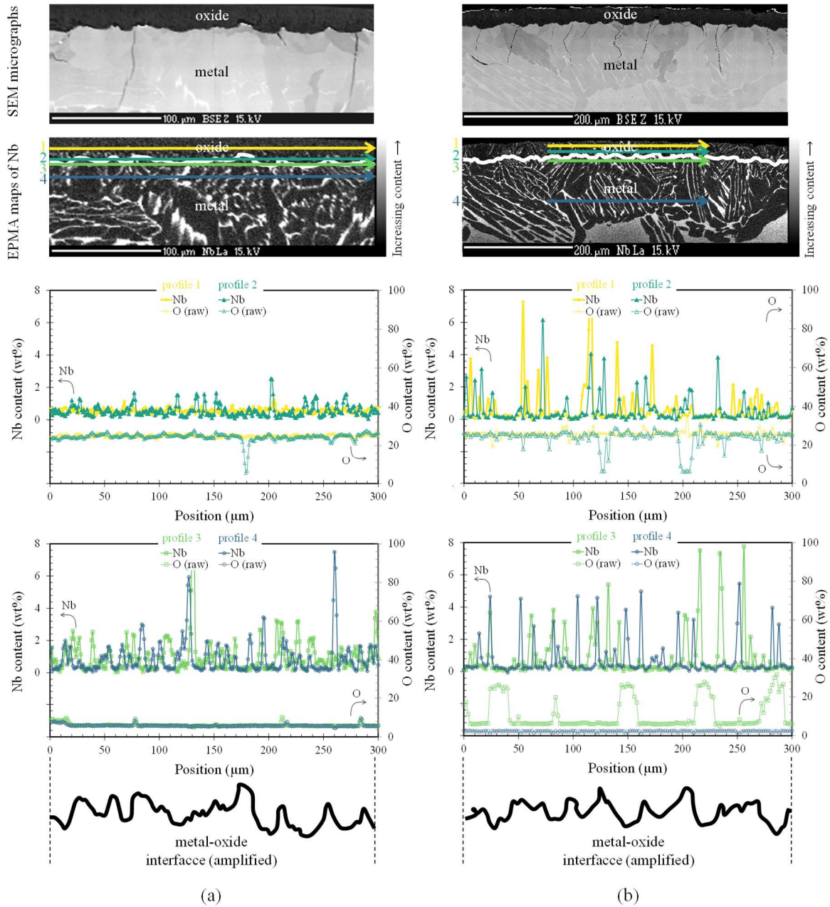
Fig. 23. SEM micrograph, EPMA X-ray map of niobium (1 pixel/ \mu\text{m} spatial resolution) and niobium and oxygen concentration along the profiles numbered 1, 2, 3 and 4 in the map of niobium (the raw data reported for oxygen overestimate the actual oxygen content values due to surface contamination which was not corrected here) along the tube hoop direction within the oxide and the metallic substrate, at a few microns from the metal-oxide interface, within a M5 Framatome (batch 1) samples (one-sided) oxidized for (a) 3270 s and (b) 7500 s at 1000°C and water quenched.
