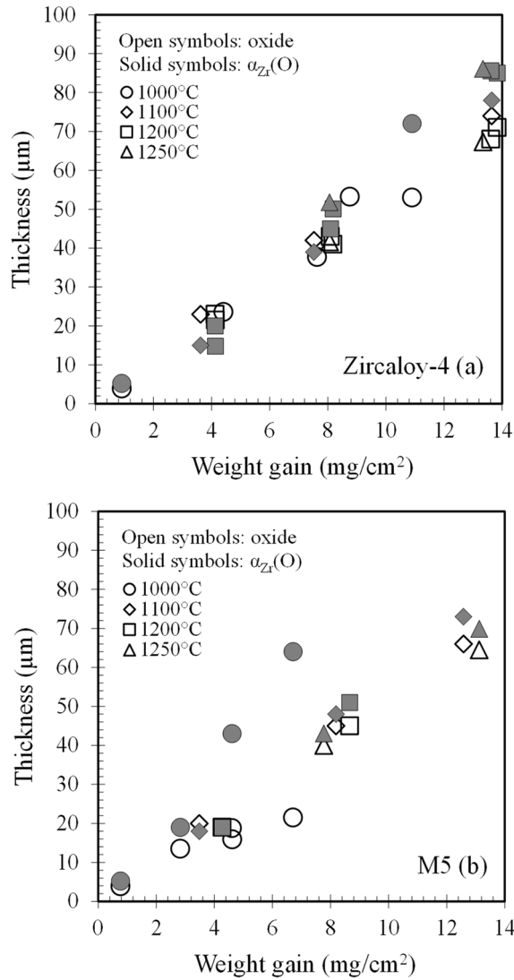
Fig. 11. Thicknesses of the oxide layer and the \alpha_{\text{Zr}}(\text{O}) layer as a function of the weight gain at 1000°C (before the onset of breakaway oxidation), 1100°C, 1200°C and 1250°C (one-side oxidation) for (a) Zircaloy-4 (batch 1) and (b) M5 Framatome (batch 1).
