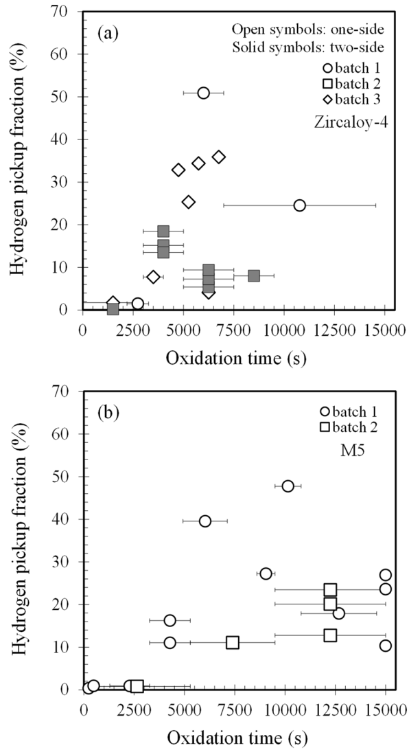
Fig. 8. Evolution of the “instantaneous” hydrogen pickup fraction (reduced to the cladding outer surface) as a function of the oxidation time under steam at 1000°C for (a) three batches of Zircaloy-4 one-sided or two-sided oxidized and (b) two batches of M5 Framatome one-sided oxidized (horizontal error bars correspond to time ranges over which the hydrogen pickup fraction has been estimated).
