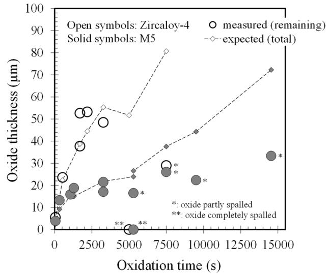
Fig. 12. Evolution of the average oxide thickness remaining at the sample surface after quenching and the total oxide thickness expected from the weigh gain (according to the data shown in Fig. 11), as a function of the oxidation time under steam at 1000°C (one-side oxidation) for Zircaloy-4 (batch 1) and M5 Framatome (batch 1).
