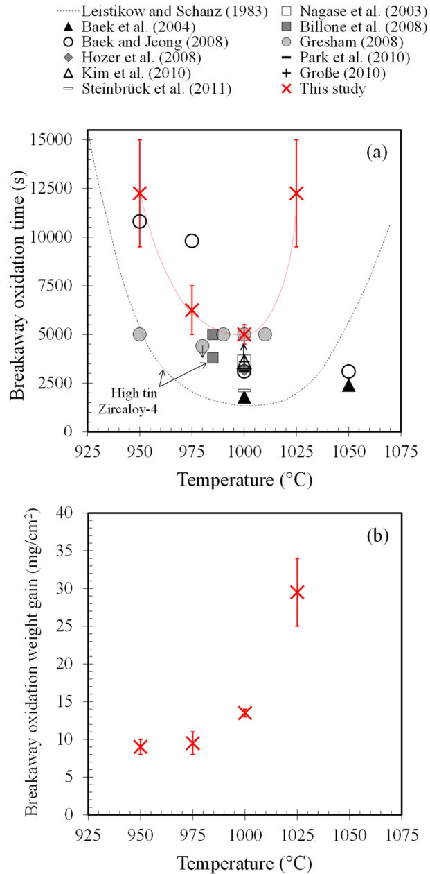
Fig. 4. Evolution of the incubation (a) time and (b) weight gain needed for breakaway oxidation of Zircaloy-4 as a function of temperature; comparison to data reported by Leistikow and Schanz [9], Nagase et al. [3], Billone et al. [11], Baek et Jeong [12], Gresham [13], Hozer et al. [14], Park et al. [15], Kim et al. [16], Große [17] and Steinbrück et al. [18].
