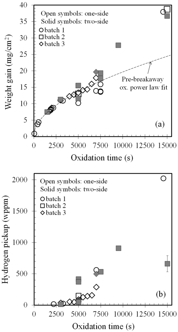
Fig. 5. Evolution of (a) the weight gain and (b) the hydrogen pickup (reduced to the cladding outer surface) as a function of the oxidation time for various batches of Zircaloy-4 one-sided or two-sided oxidized under steam at 1000°C.
