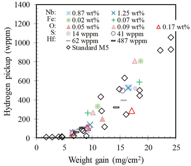
Fig. 10. Evolution of the hydrogen pickup as a function of the weight gain at 1000°C (one-side oxidation) for standard M5 Framatome and materials with chemical compositions (various contents of Nb, Fe, O, S and Hf) around the nominal specifications of M5 Framatome .
