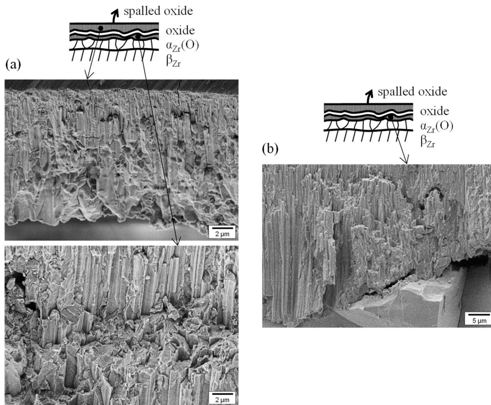
Fig. 19. FEG-SEM fractographs of fragments of oxide spalled during quenching of M5_{\text{Framatome}} (batch 1) samples fractured at room temperature after one-side oxidization for (a) 9500 s and (b) 14551 s at 1000°C and water quenching.
