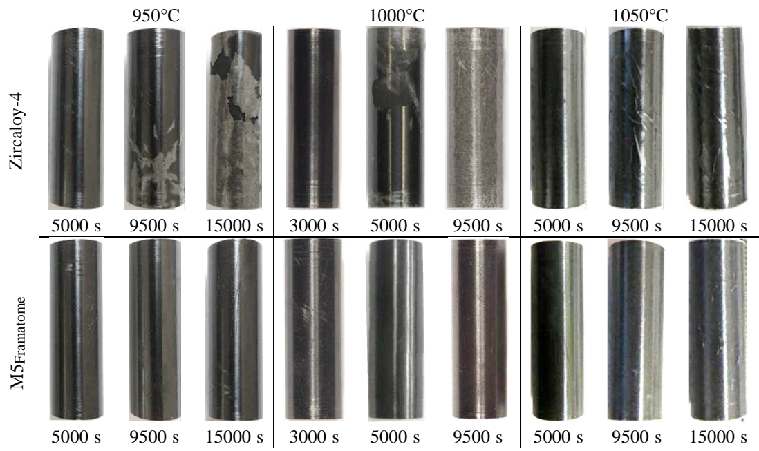
Fig. 3. Post-quenching appearance of Zircaloy-4 (batch 2) and M5 Framatome (batch 2) cladding specimens two-sided oxidized in steam at 950, 1000 and 1050°C.
