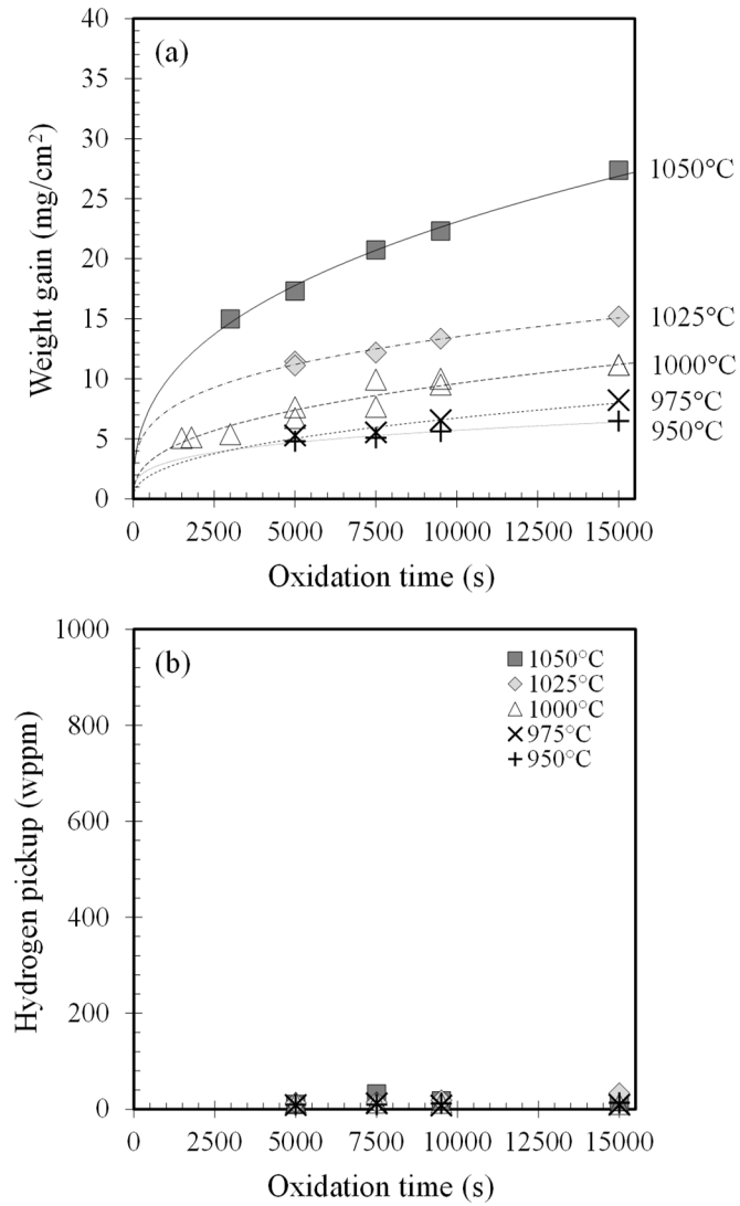
Fig. 2. Evolution of (a) the weight gain (the trend lines follow power laws) and (b) the hydrogen pickup (reduced to the cladding outer surface) as a function of the oxidation time under steam at 950, 975, 1000, 1025 and 1050°C (two-side oxidation) for M5 Framatome (batch 2).
