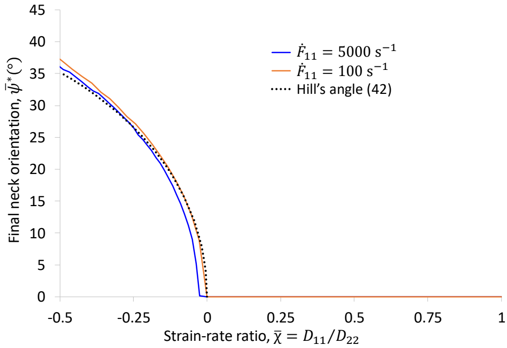
Fig. 5. (a) Evolution of the critical initial imperfection orientation with the loading path parameter.
