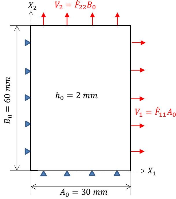
Fig. B.1. Illustration of the configuration considered in the finite element computations of plate necking.
