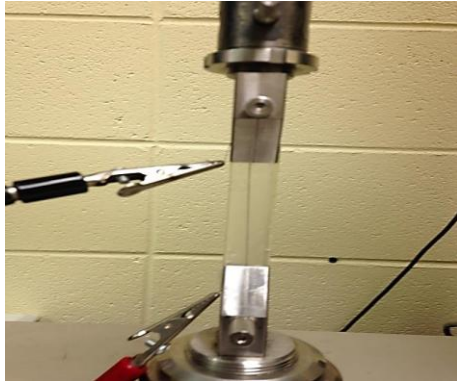
Fig.6. Composite sample placed in the machine with sensor attached to the oscilloscope
