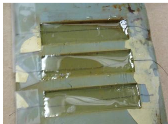
Fig.5. Sensor wire integrated with in the composite specimen
