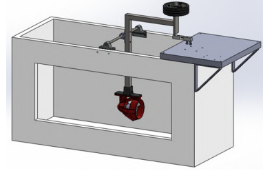
Fig. 11. Test bench used for identification
