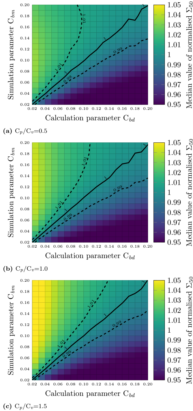
Fig. 14. Effect of the step size (with the C_p/C_v ratio) on the median value mappings of \Sigma_{50} distribution determined using 1000 simulated staircases of n = 100 specimens - Sensitivity of the C_{bd} parameter on the fatigue strength calculation method using an initial distribution with C_v=0.1
