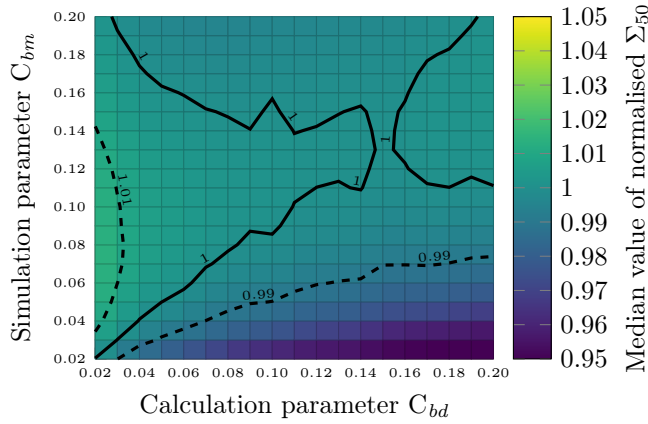
(a) Mapping of the median values of \Sigma_{50} distributions
