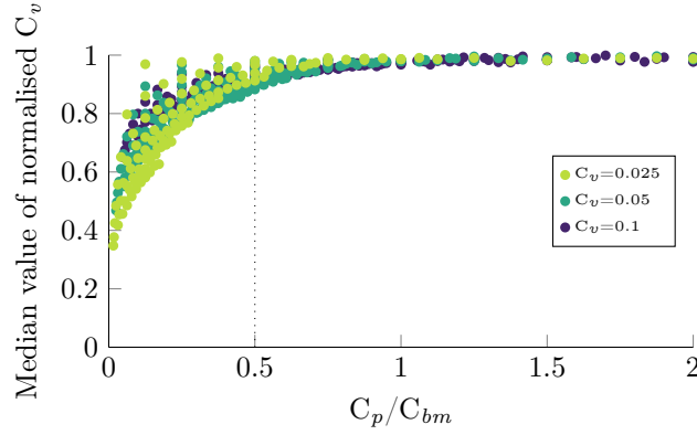
Fig. 11. Effect of the C_p/C_{bm} ratio on the median value of the coefficient of variation distributions determined using 1000 simulated staircases of n = 100 specimens and the interval censoring method - Comparison for three initial distributions using various step sizes C_p and simulation parameters C_{bm}
