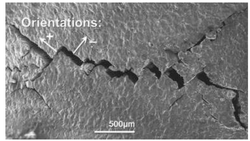
Figure 7. A closer view of the load-level 2 sample surface shown in Fig 6d.
