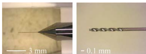
Figure 2. Titanium drill of diameter 0.1 mm.
