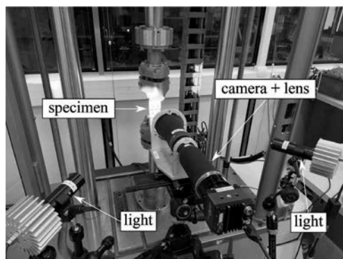
Figure 3. Experimental device.
