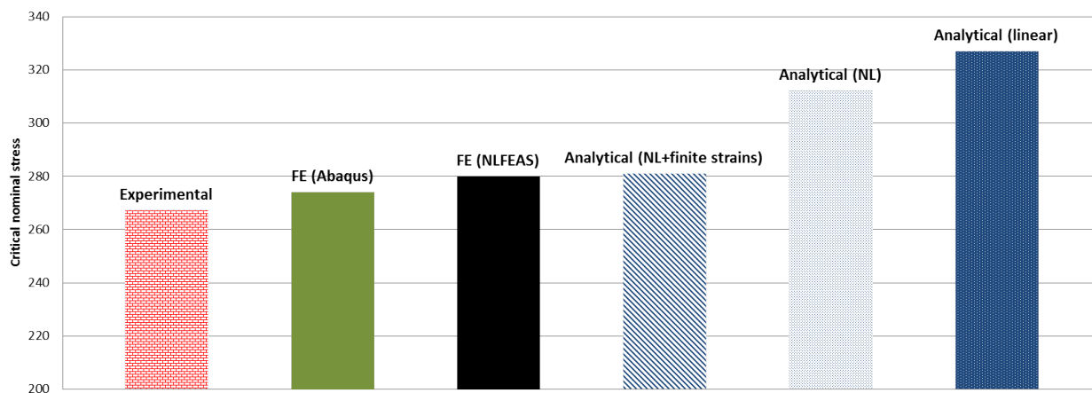
Figure 12: Comparison between analytical, numerical and experimental critical stresses
