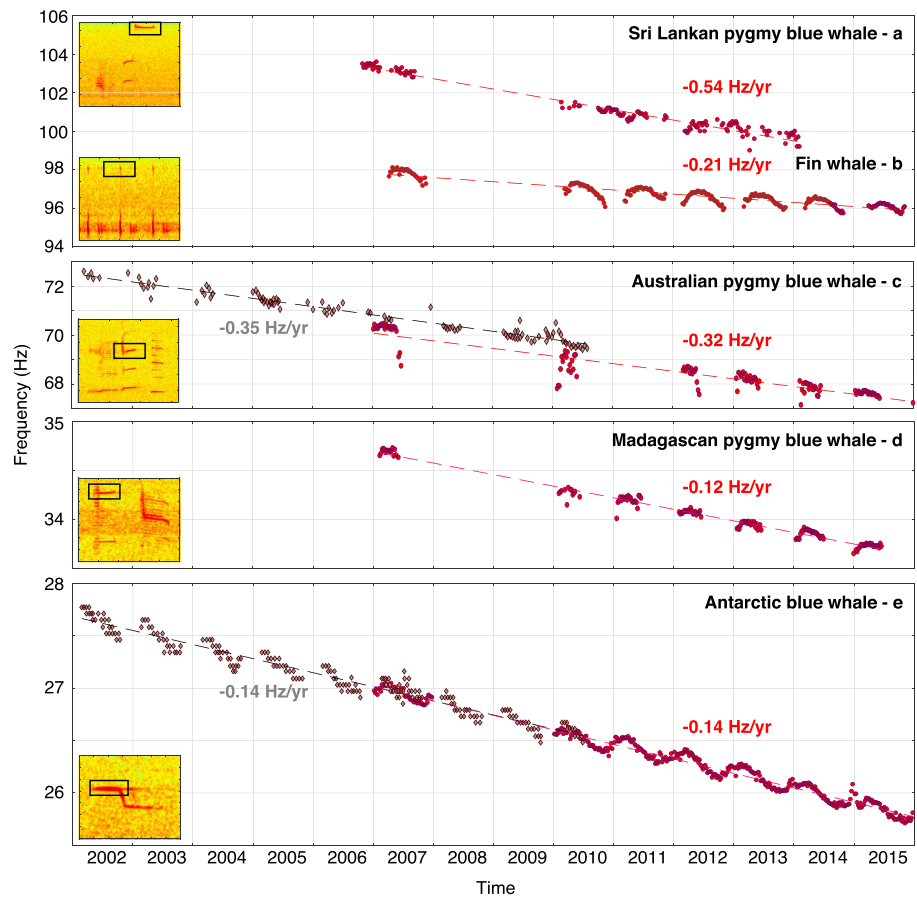
Figure 3. Fin and blue whale call-frequency decline over the years in the southern Indian Ocean. Symbols (red, this study; black diamonds, data digitized from Gavrillov et al., 2012) are weekly averaged peak frequencies measured for selected units in the calls (black rectangles in the time-frequency diagrams). The rates of frequency decrease in hertz per year are the slopes of the fitted dashed lines. Spectrogram insets are zoomed-in in Figure 2.
