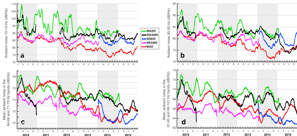
Figure 4. Long-term decrease of the ambient noise level in the (a) 10- to 13-Hz, (b) 30- to 33-Hz, (c) 64- to 66-Hz and 71- to 73-Hz, and (d) 91- to 93-Hz and 99- to 101-Hz frequency bands at all sites except the north of Crozet Island. Frequency bands (a) and (b) bracket the Antarctic blue whale calls, (c) the Australian pygmy blue whale calls, and (d) the 99-Hz fin whale pulses. MAD = Madagascar Basin; NEAMS = northeast of Amsterdam Island; SSEIR = northern Crozet Basin; SWAMS = between Kerguelen and Amsterdam islands; WKER = between Crozet and Kerguelen islands.
