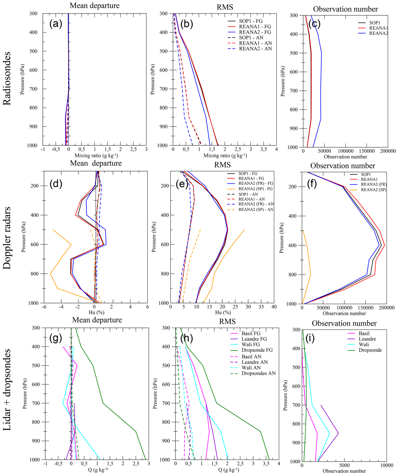
Figure 8. First-guess (FG, solid lines) and analysis (AN, dashed lines) departure against radiosounding (mixing ratio, g kg -1 ) (a–c), against humidity derived from Doppler radar (humidity, percent) (d–f), and against lidars and dropsondes (mixing ratio, g kg -1 , only for REANA2) (g–i); columns correspond to mean departure (a, d, g), root mean square departure (b, e, h), and observation numbers (c, f, i). In panels (a–g), black curves are for SOP1, red is for REANA1, and blue is for REANA2. Orange lines are for Spanish radars in REANA2. Computation period extends from 5 September 2012 to 5 November 2012.
