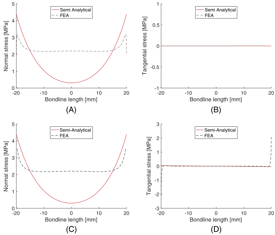
FIGURE 8 Stress distribution along the adhesive layer for the DNS Arcan specimen loaded at 0^\circ : A and B, Mid-thickness of the bond line. C and D, Adhesive/substrate interface [Colour figure can be viewed at wileyonlinelibrary.com ]
