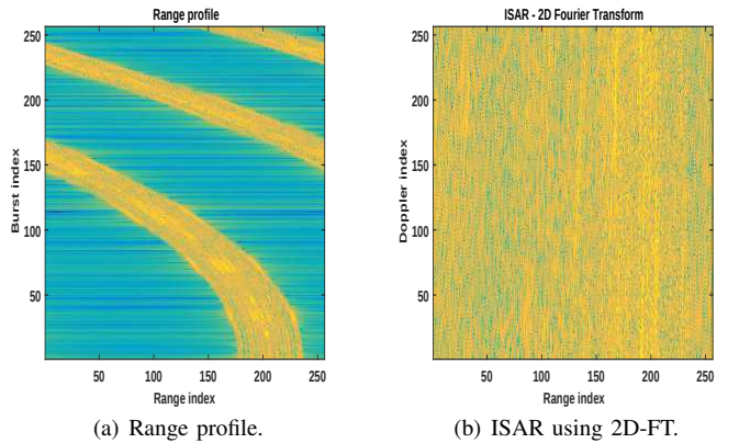
Fig. 9. Range profile and ISAR image of uncompensated target.
