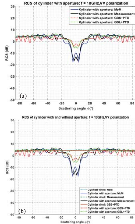
Fig. 7. (a) Measured and simulated RCS of a hollow circular cylinder with an aperture, (b) RCS of a cylinder with and without an aperture.
