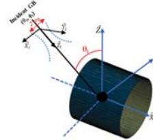
Fig. 1. Geometric configuration of a cylinder illuminated by incident Gaussian Beam (GB), width ( 2\omega_0 ).
