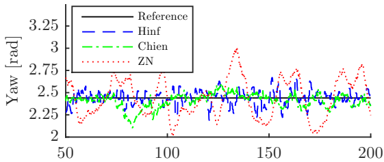
Fig. 10. Perturbation at 45^\circ of surge direction
