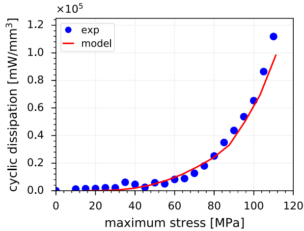
Fig. 17 Comparison between the cyclic dissipated evaluated from the model and measured
