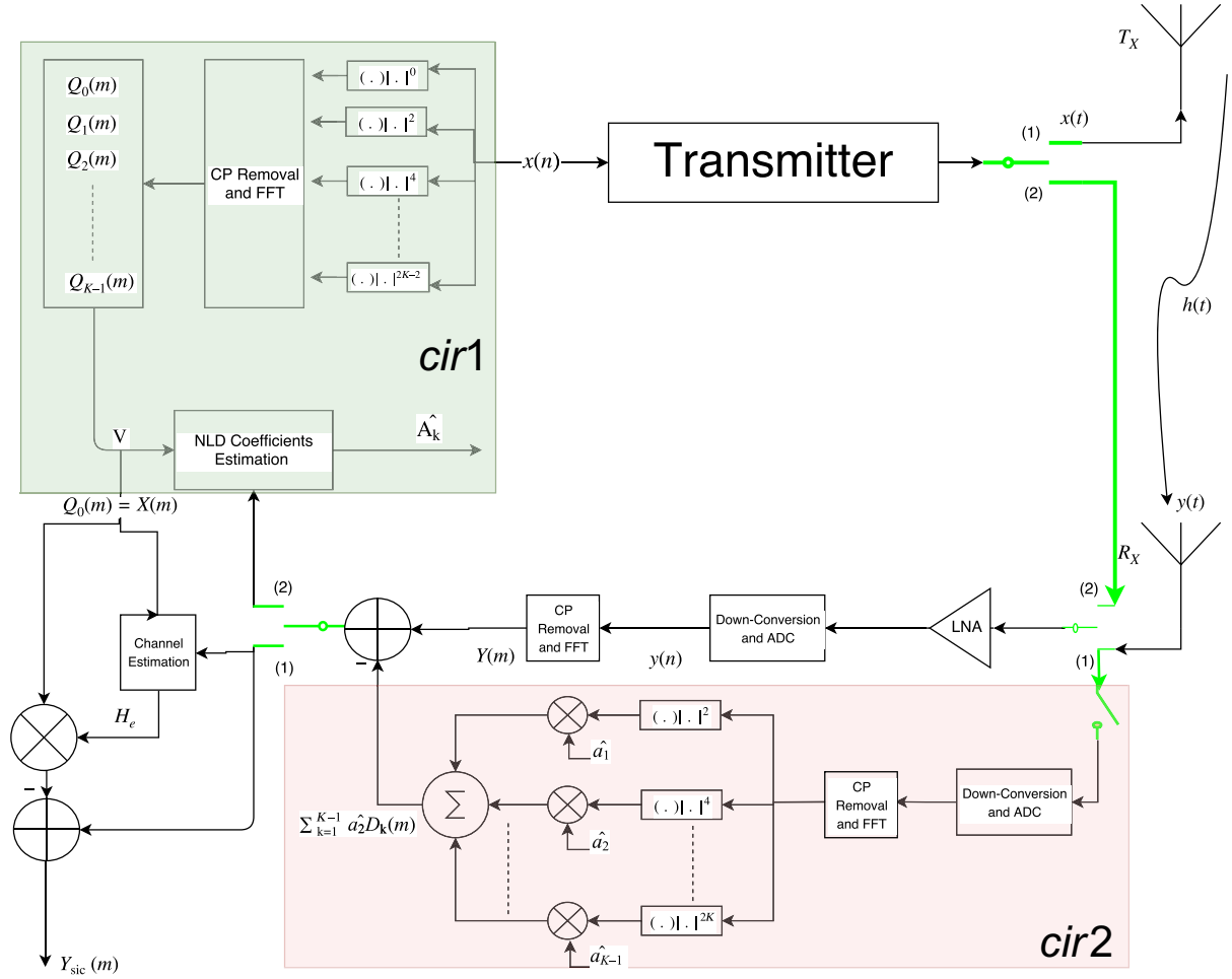
FIGURE 2 A full-duplex system capable to reduce the nonlinear distortion (NLD) of the receiver low-noise amplifier (LNA). The circuit cir1 (green color) stands for the estimation of the NLD coefficients using a wire in order to avoid the effect of the wireless channel, in this case, the switches are on position (2). When the switches are on the first position (1), the transceiver works in ordinary conditions, and the circuit cir2 (pink color) helps in reducing the NLD before estimating the channel. ADC, analog-to-digital converter; CP, cyclic prefix; FFT, fast Fourier transform
