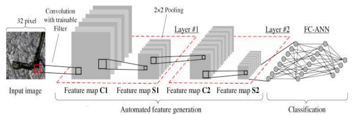
Fig. 1. CNN architecture.
