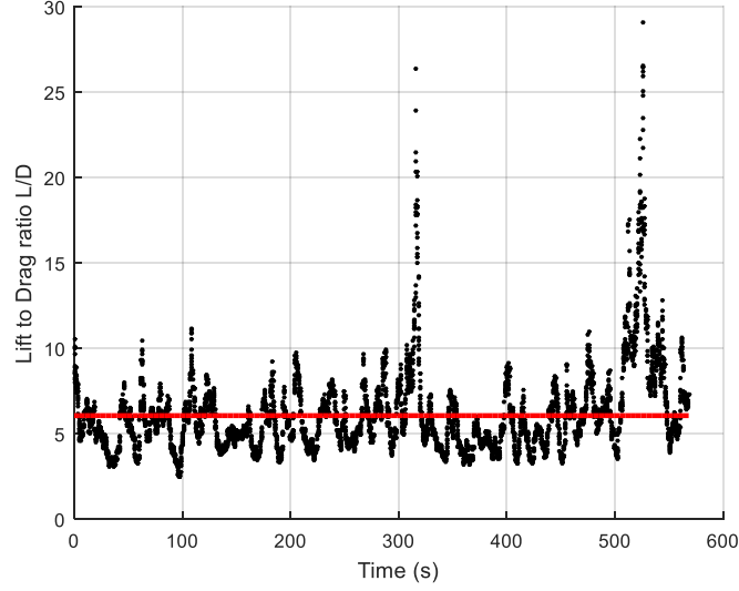
Fig. 7: Lift to drag ratio for each point using Eq. (11) (dotted), during a 569s run with kite in static flight. The solid red line is the mean of the lift to drag ratio during the considered period, and is equal to 6.06. The associated standard deviation is 2.45.
