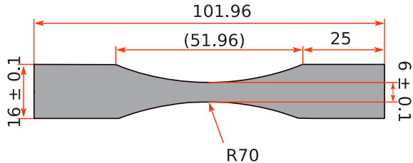
Fig. 13. Shape of the used specimens to observe deformation mechanisms.
