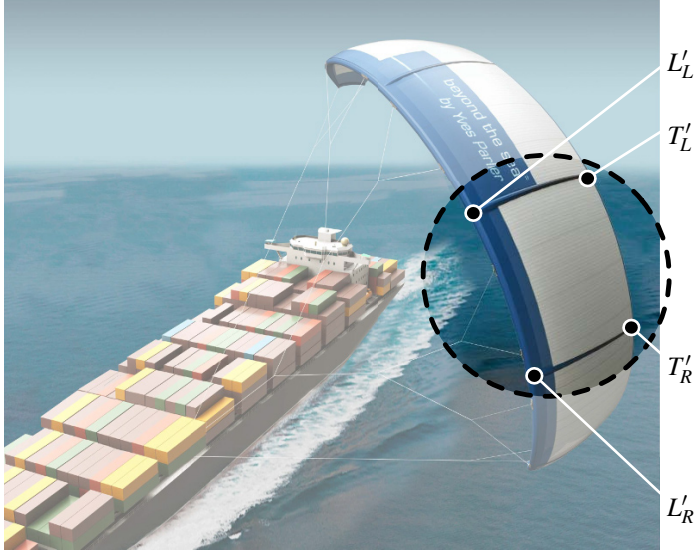
Fig. 4.2 A representative elementary cell with corner points L'_L, L'_R, T'_R and T'_L which are located at the extremities of the inflatable battens
