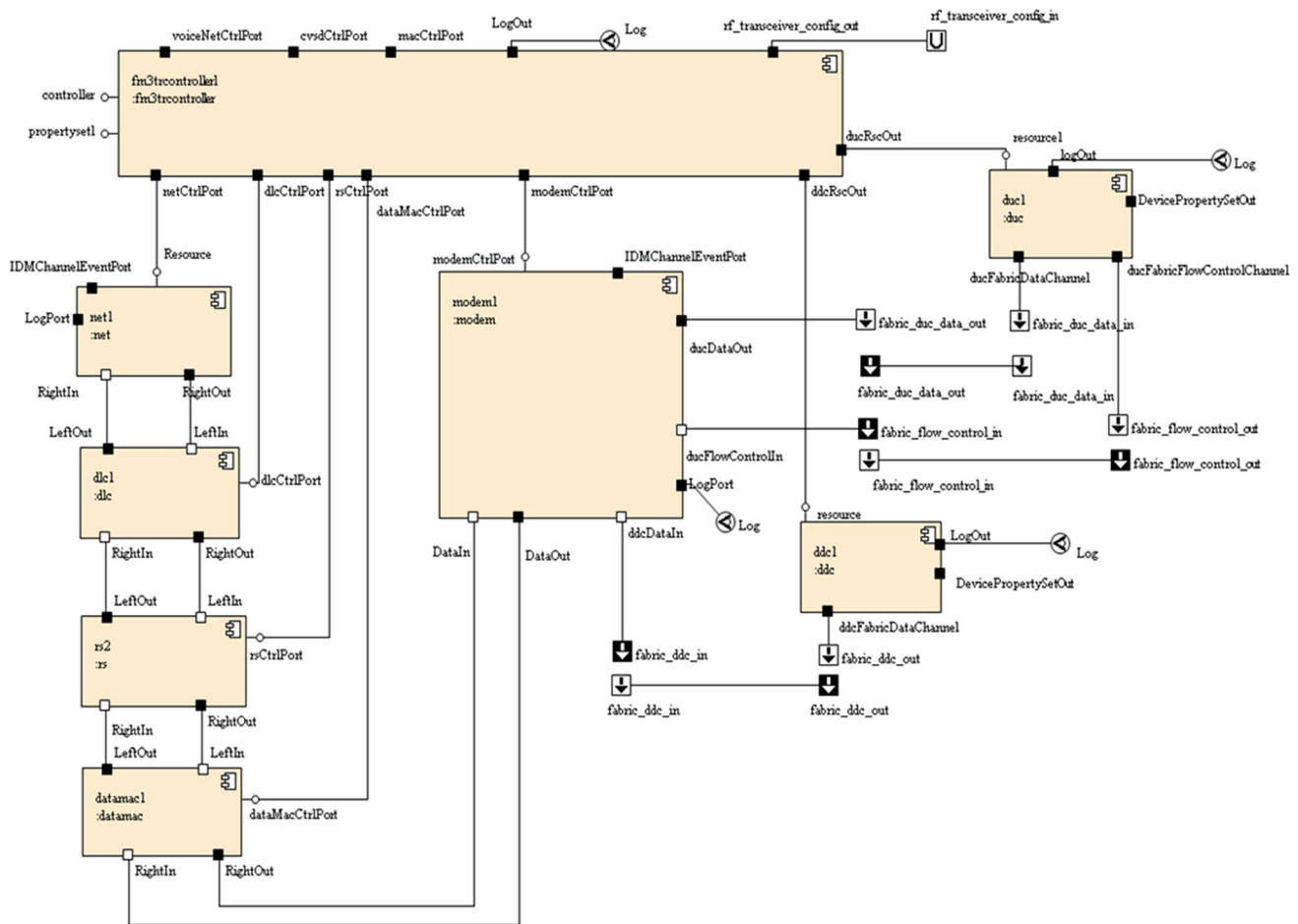
Fig. 7 FM3TR waveform deployment in an SDR-3002
