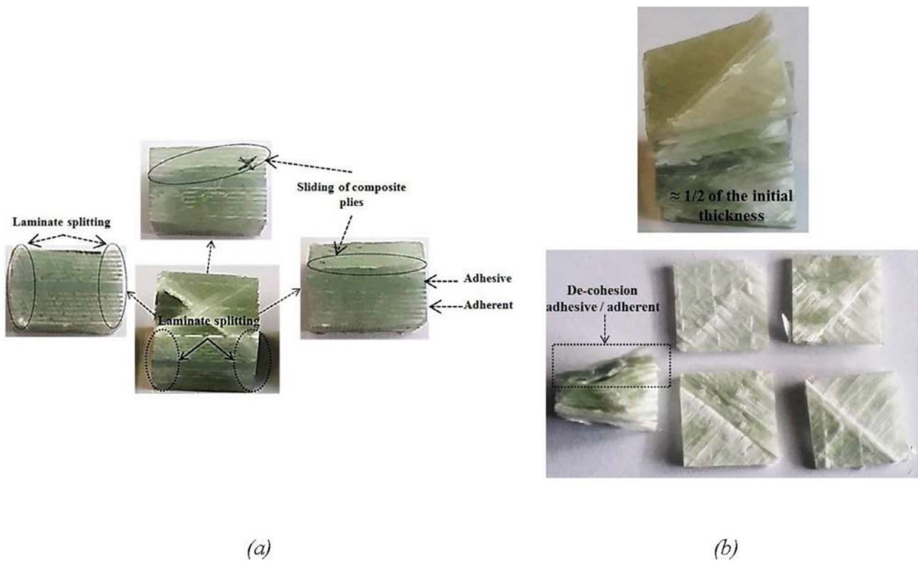
Fig. 8. Cross-sectional views of specimens tested at (a) 312 \text{ s}^{-1} and at (b) 713 \text{ s}^{-1} .
