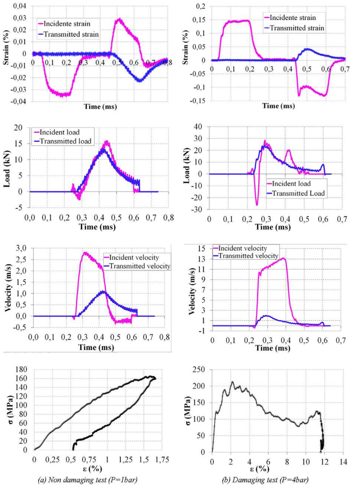
Fig. 3. Typical results of signal processing from gauges.
