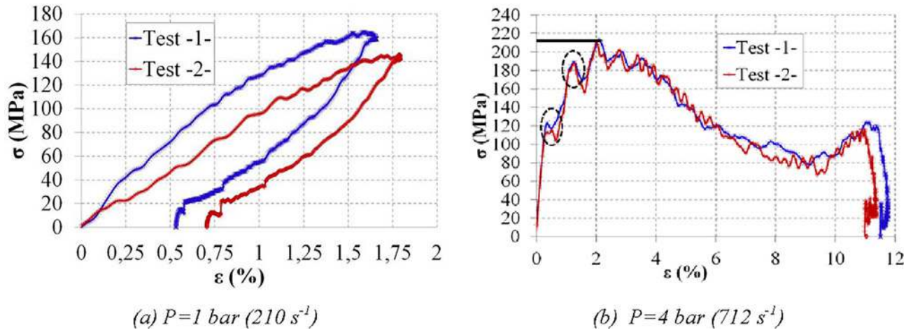
Fig. 5. Test reproducibility for IP tests.
