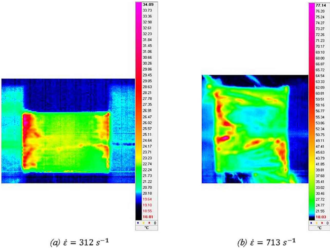
Fig. 13. Heating of the sample during damage.
