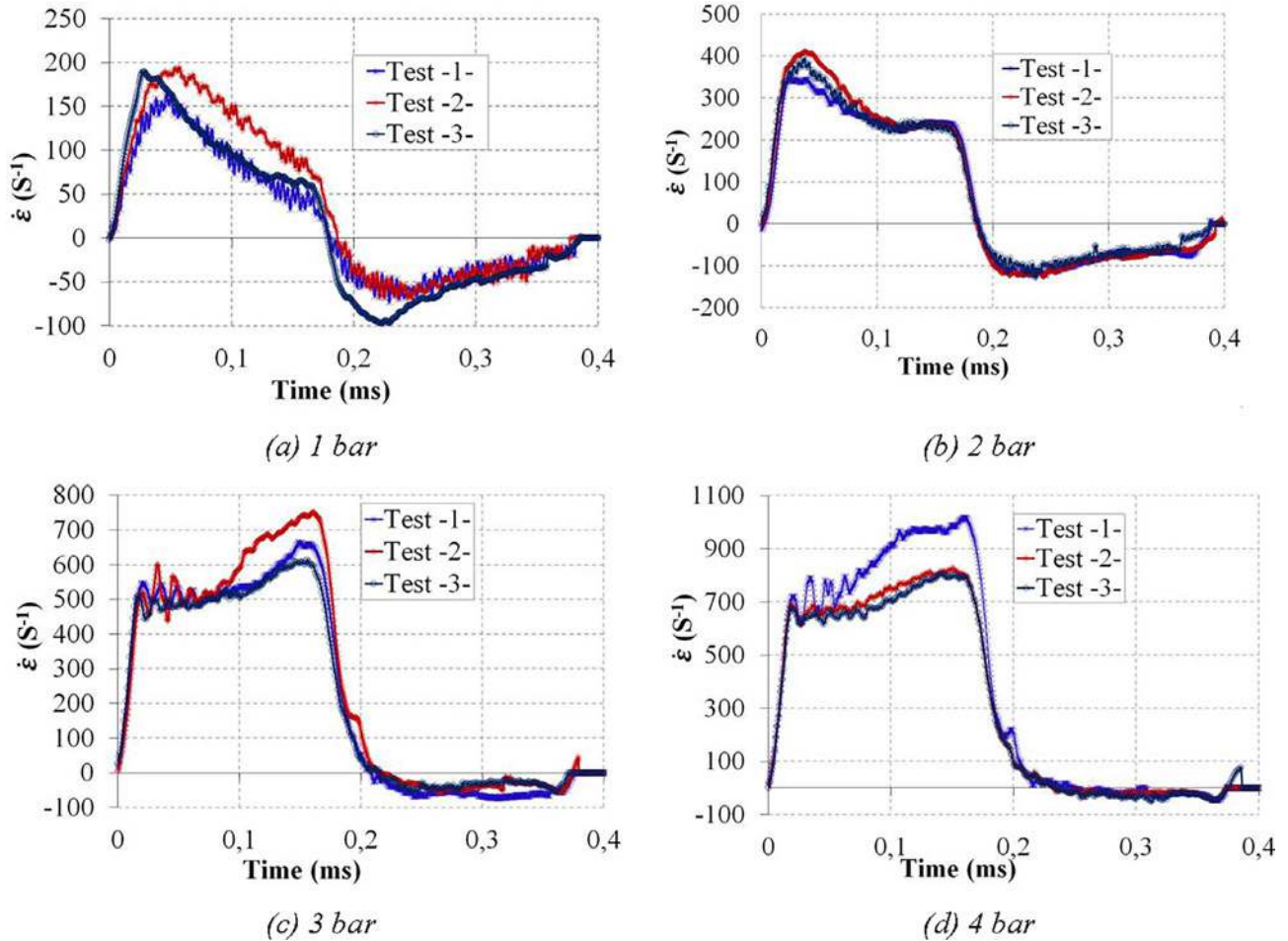
Fig. 4. Test reproducibility of strain rate evolution vs. time for impact pressure.
