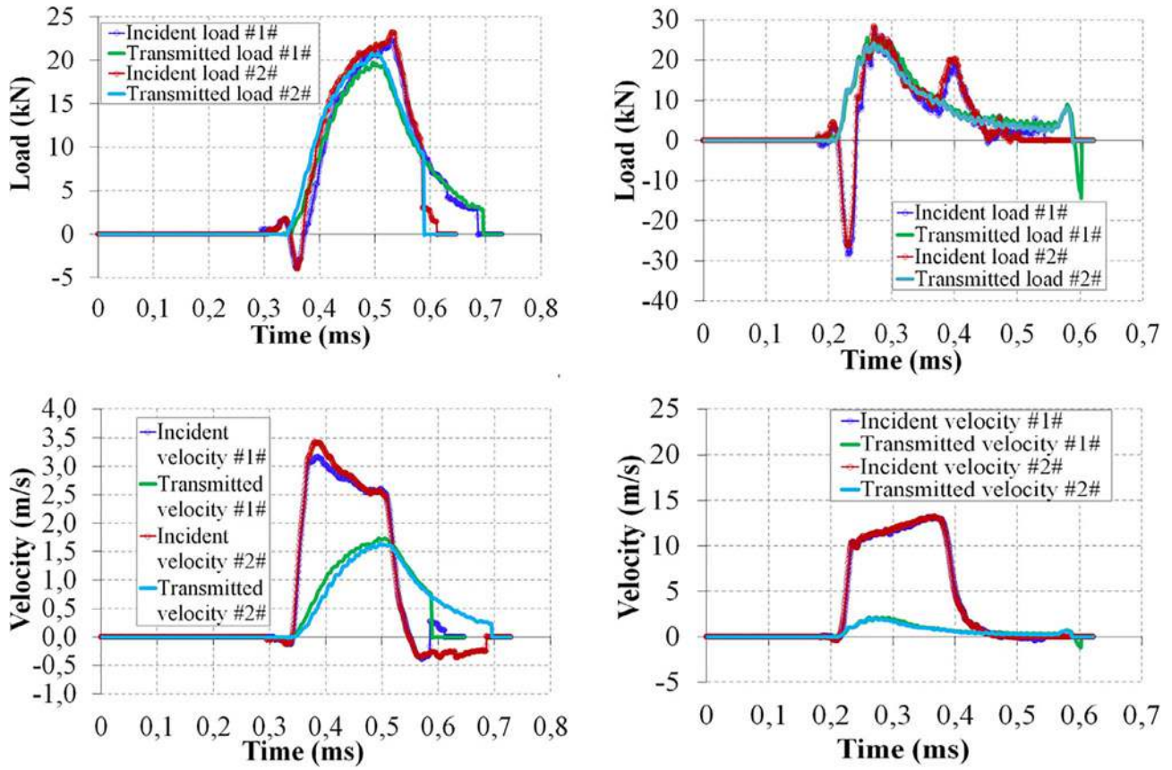
(a) Non damaging test, 210 \text{ s}^{-1}
