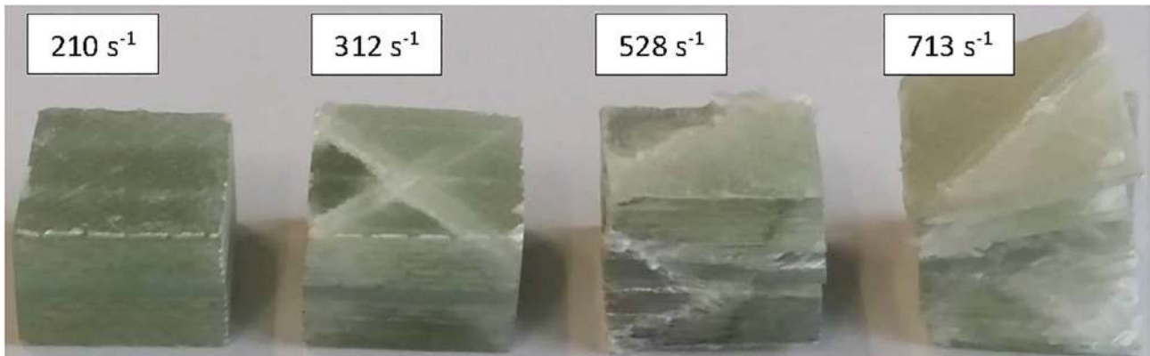
Fig. 11. Recovered specimens after IP dynamic compression tests.
