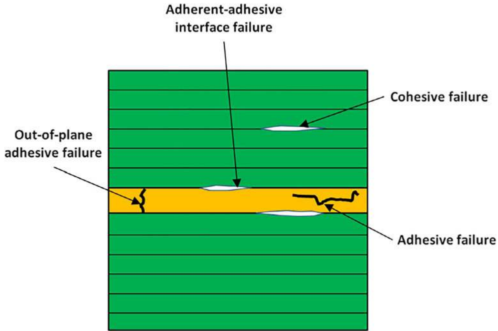
Fig. 10. Typical failure modes of an adhesively bonded composite joint.
