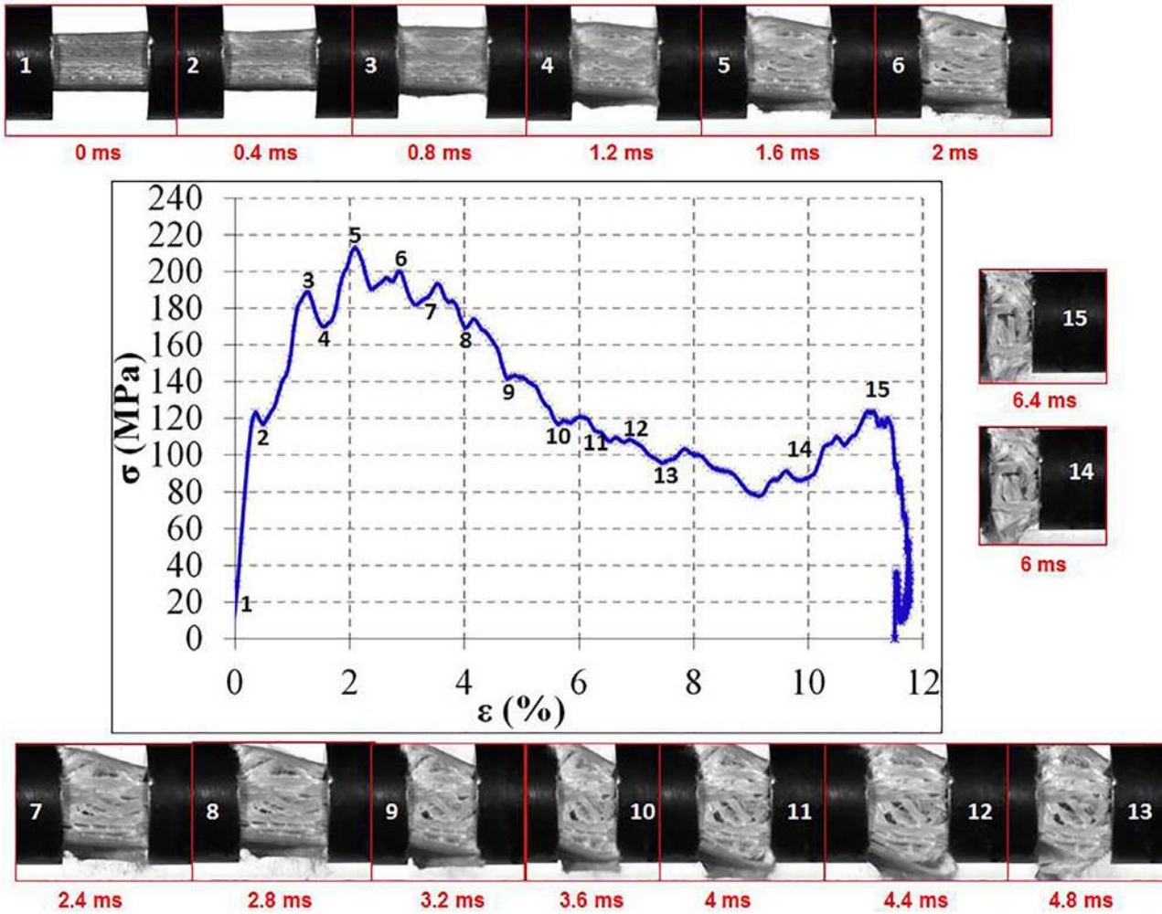
Fig. 12. High speed photograph of real-time dynamic compression test of adhesively bonded joints impacted at high strain rate of 713 \text{ s}^{-1} .
