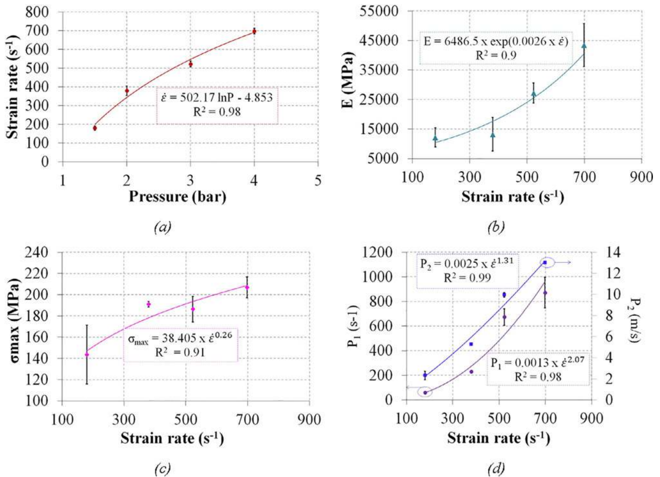
Fig. 9. Strain rate vs pressure, E , \sigma_{max} , P_1 and P_2 vs strain rate evolutions.
