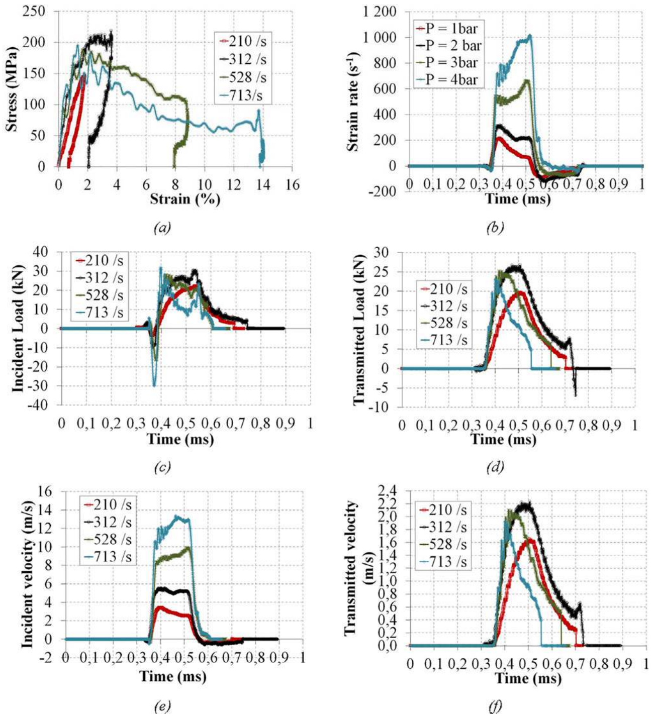
Fig. 7. Dynamic parameters for different impact pressures.
