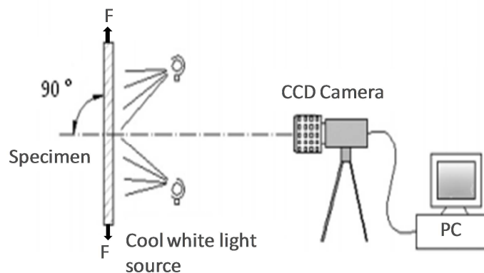
Fig. 2. Schematic experimental set-up
