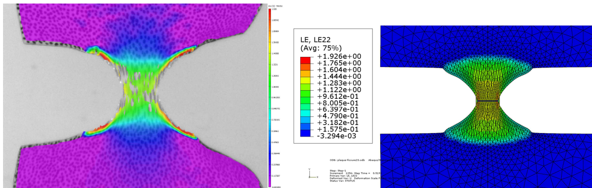
(DIC/maximum displacement = 15.57 mm)
