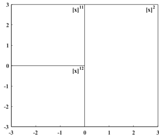
Figure 3: Bisectioning the box [x] yields the boxes [x]^1 and [x]^2 . Bisectioning [x]^1 creates the boxes [x]^{11} and [x]^{12} .
