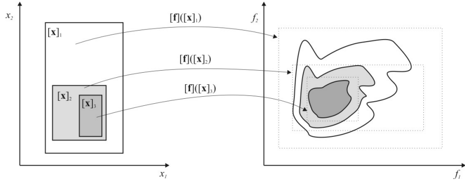
Figure 5: An example of a convergent monotonic inclusion function [23]
